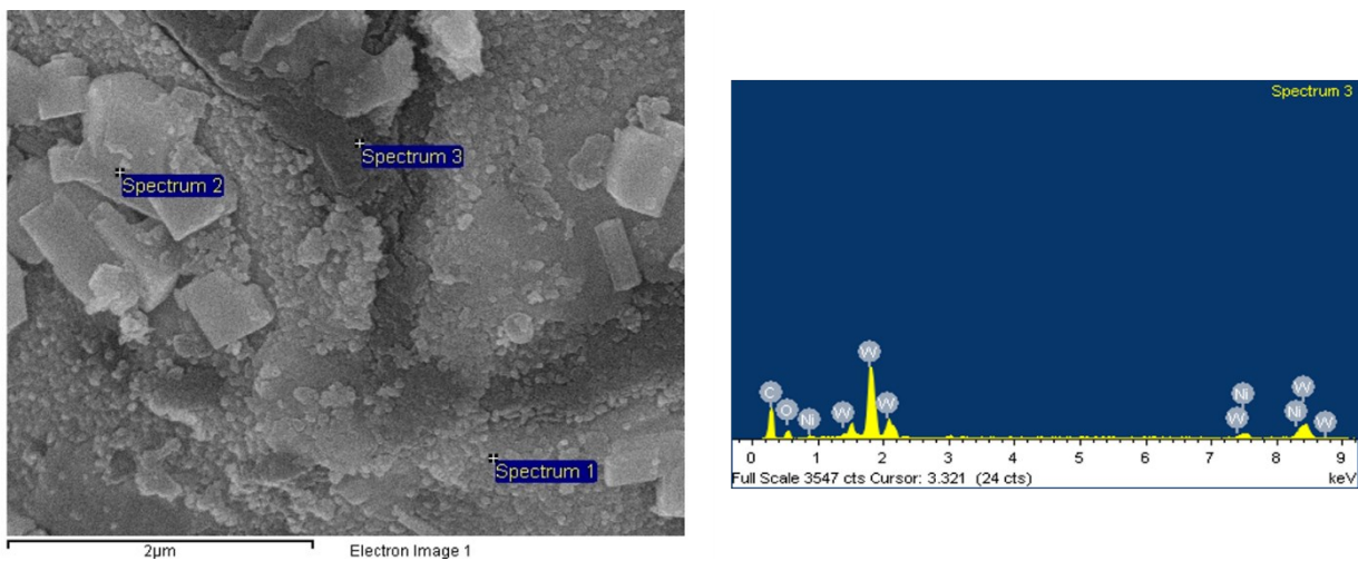
Fig. S1 The elemental surface analysis for NiW/AC catalyst.
