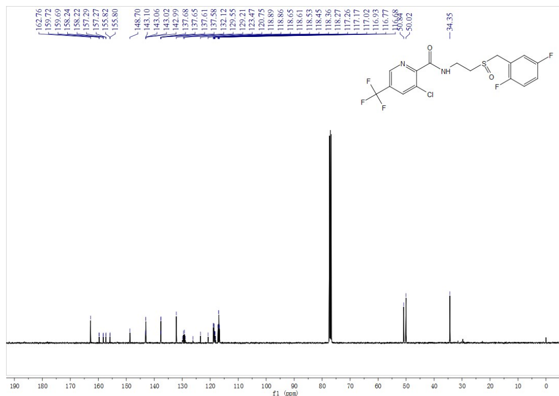
Fig. S155 13 C NMR spectra of compound G16
