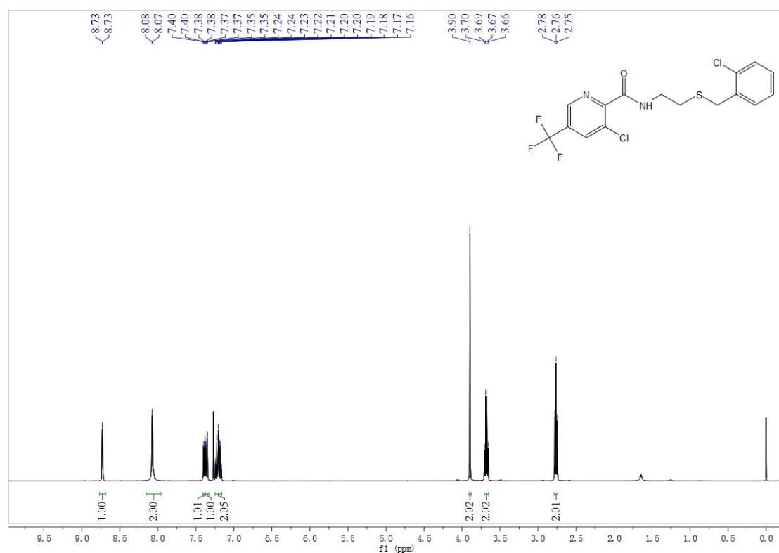
Fig. S55 1 H NMR spectra of compound E19
