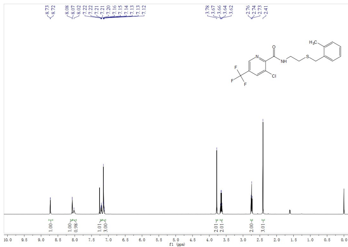
Fig. S49 1 H NMR spectra of compound E17
