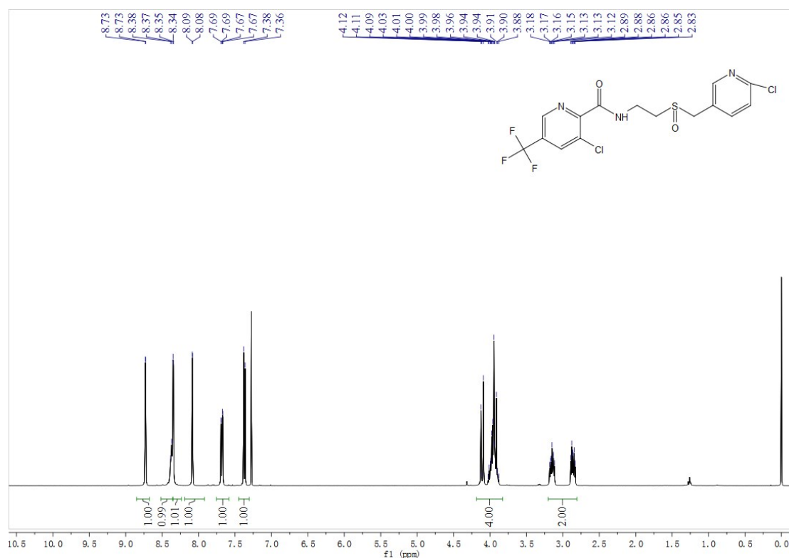
Fig. S139 1 H NMR spectra of compound G11
