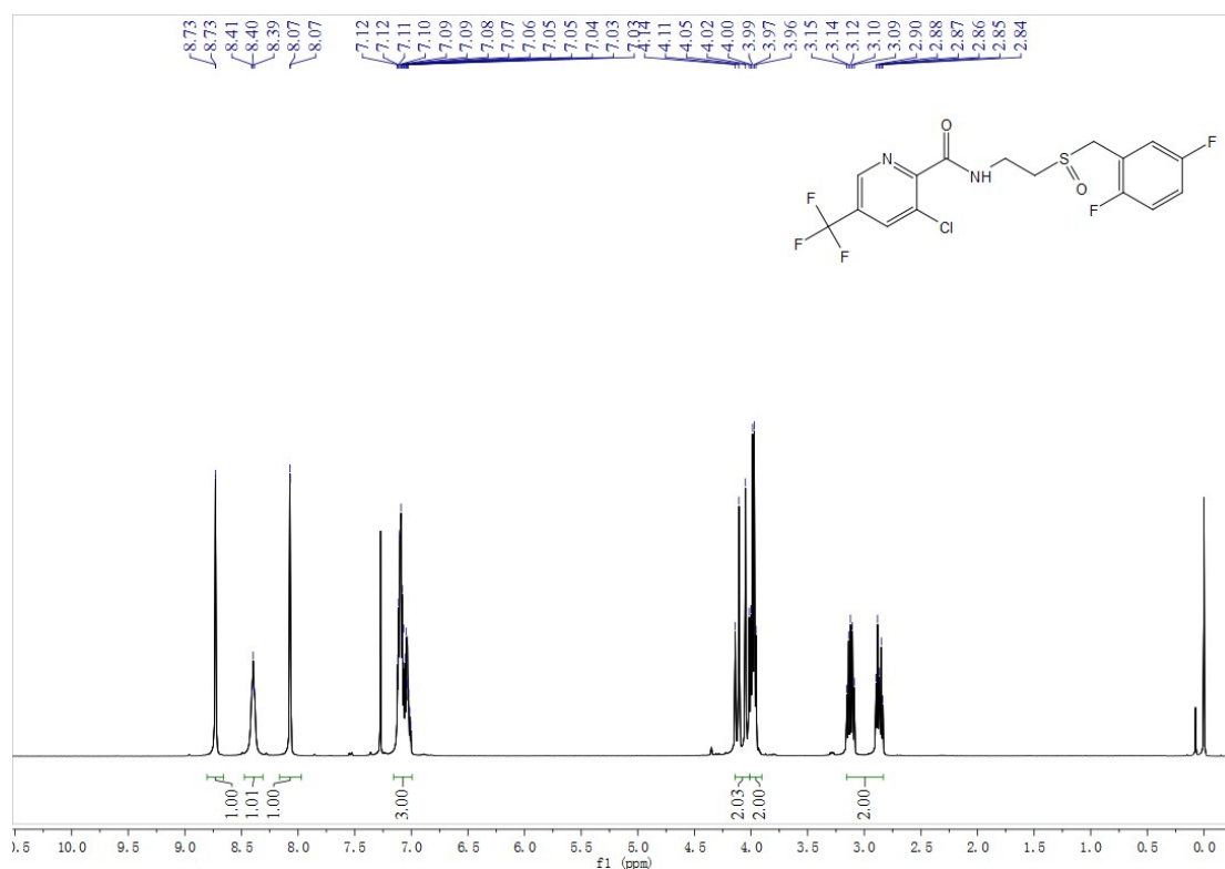
Fig. S154 1 H NMR spectra of compound G16
