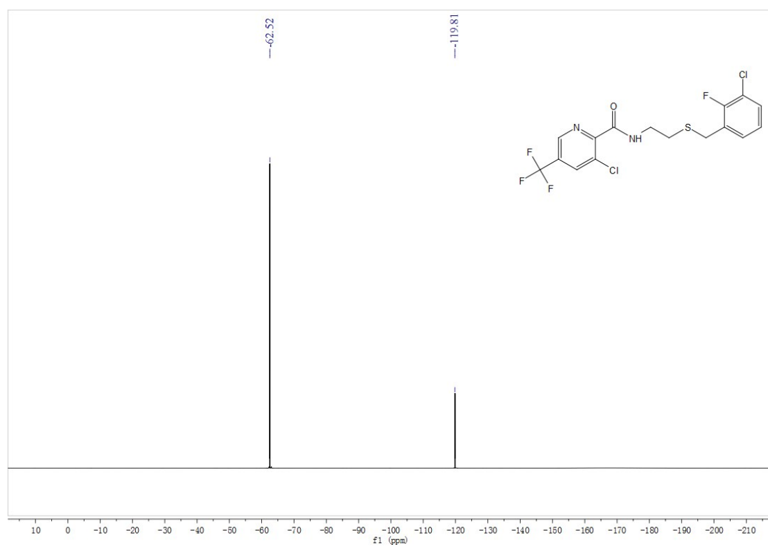
Fig. S21 ^{19}\text{F} NMR spectra of compound E7
