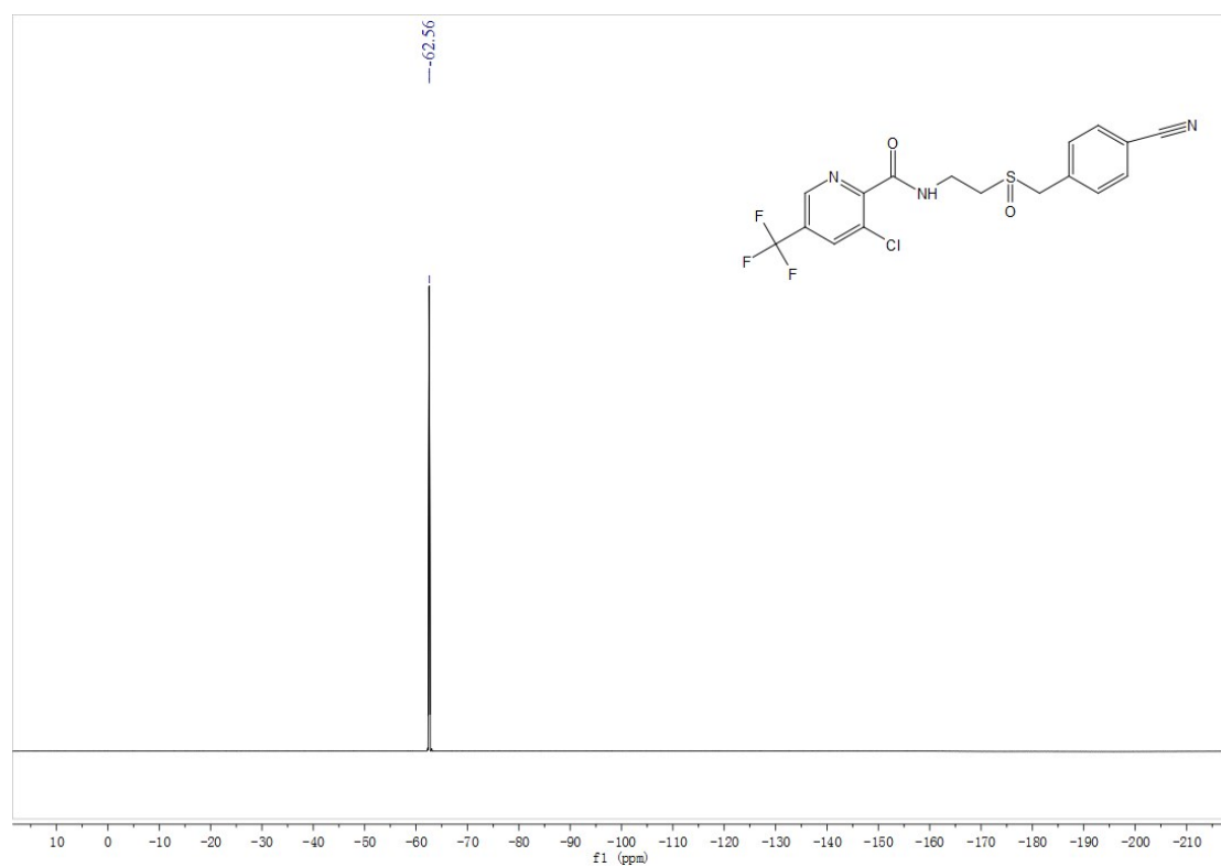
Fig. S144 ^{19}\text{F} NMR spectra of compound G12
