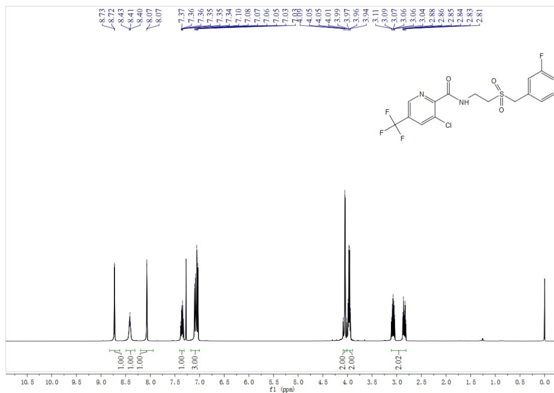
Fig. S91 1 H NMR spectra of compound F5
