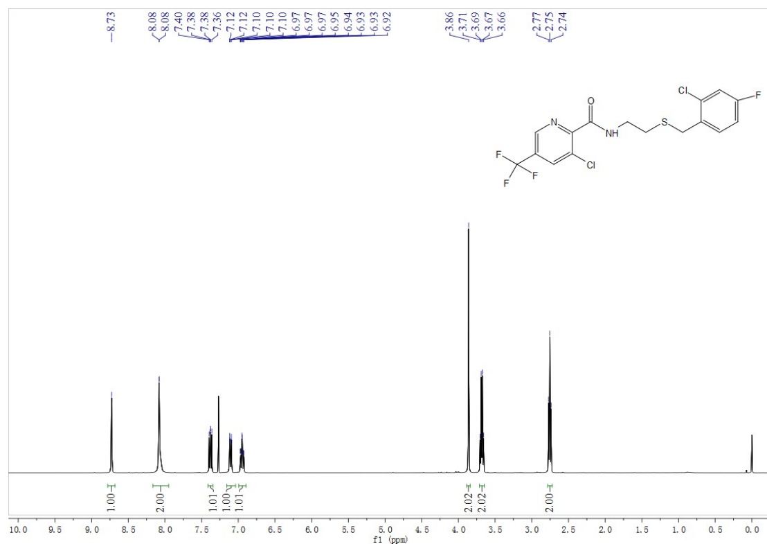
Fig. S34 1 H NMR spectra of compound E12
