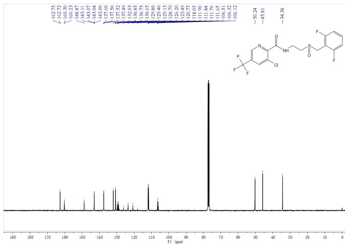
Fig. S125 13 C NMR spectra of compound G6
