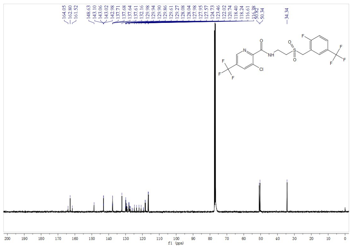
Fig. S83 13 C NMR spectra of compound F2
