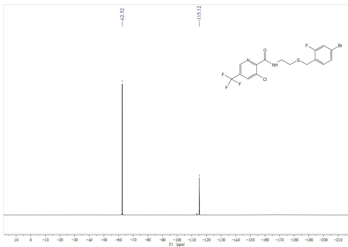
Fig. S9 ^{19}\text{F} NMR spectra of compound E3
