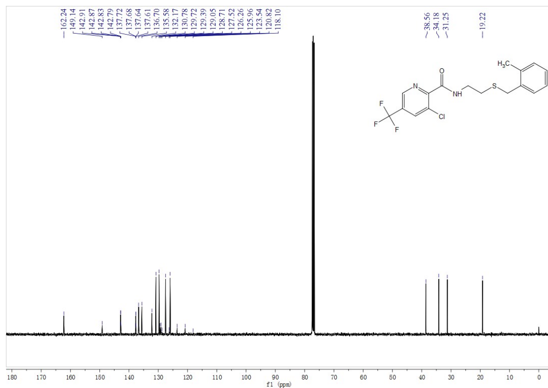
Fig. S50 13 C NMR spectra of compound E17
