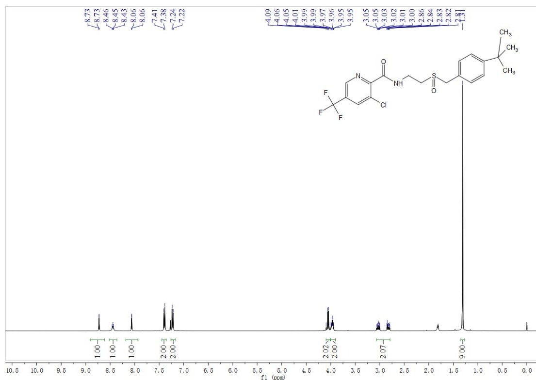
Fig. S136 1 H NMR spectra of compound G10
