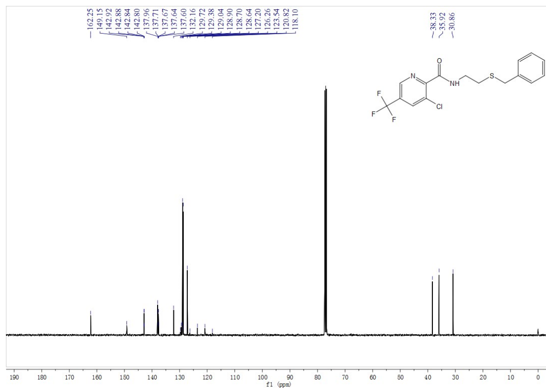
Fig. S26 13 C NMR spectra of compound E9
