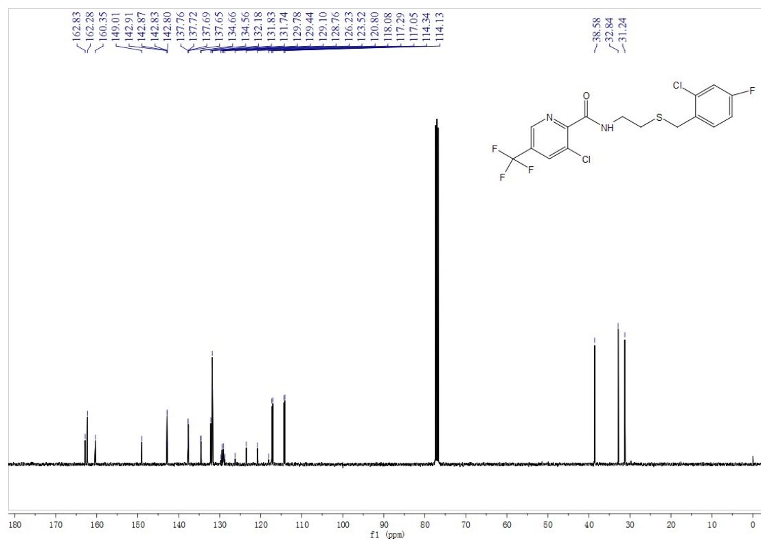
Fig. S35 13 C NMR spectra of compound E12
