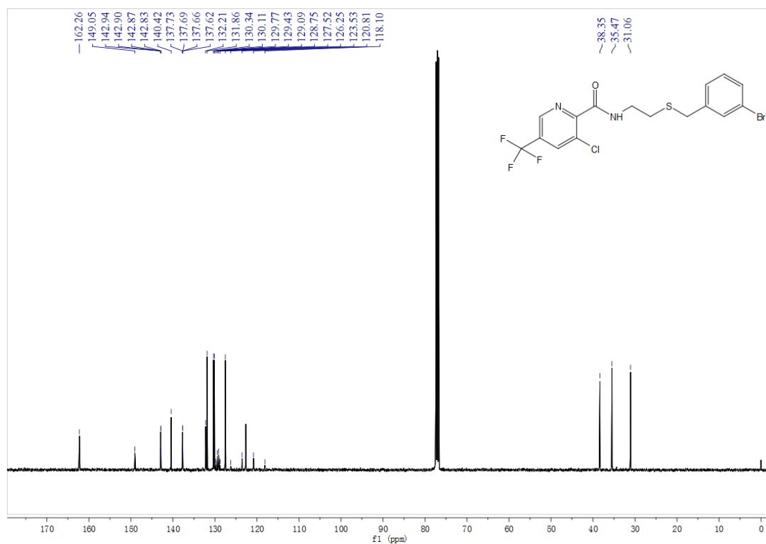
Fig. S44 13 C NMR spectra of compound E15
