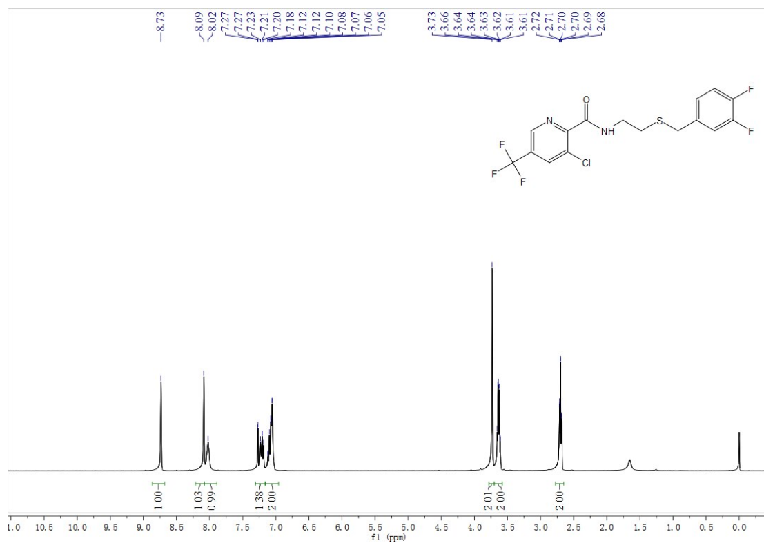
Fig. S22 1 H NMR spectra of compound E8
