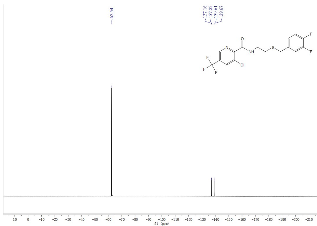
Fig. S24 ^{19}\text{F} NMR spectra of compound E8
