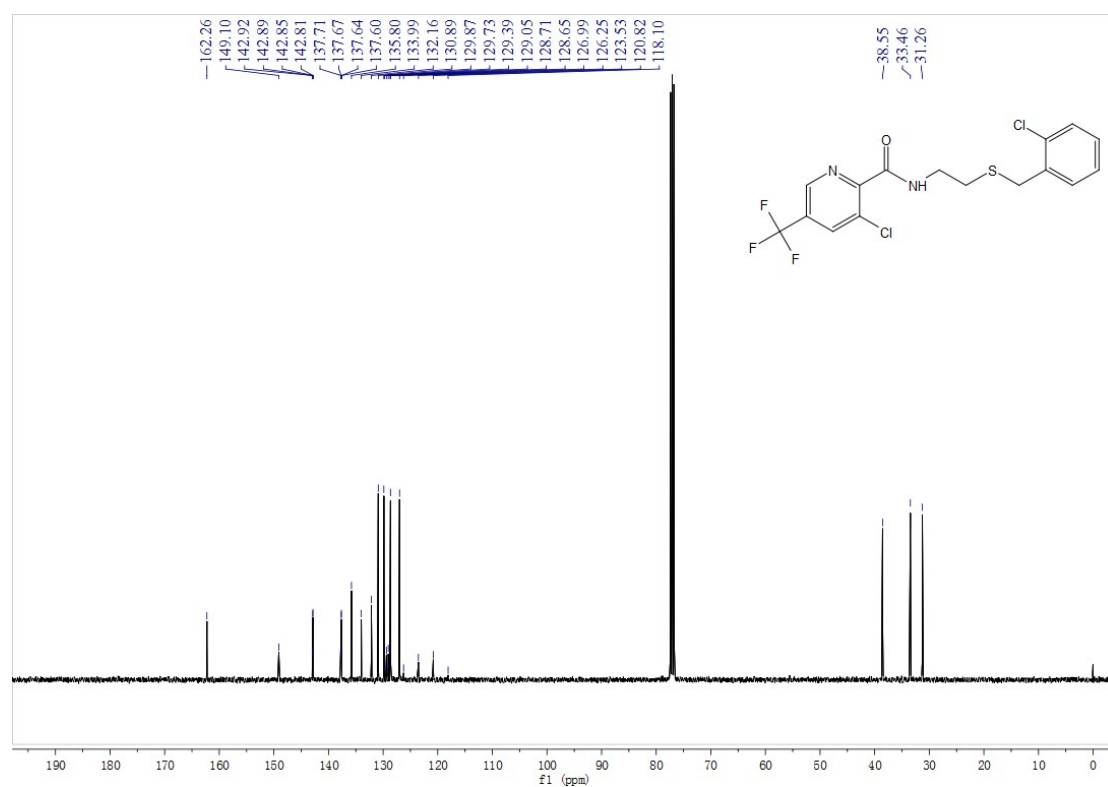
Fig. S56 13 C NMR spectra of compound E19
