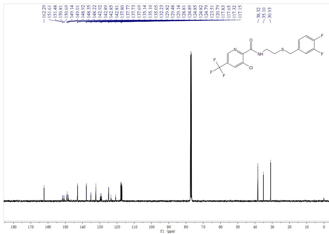
Fig. S23 13 C NMR spectra of compound E8
