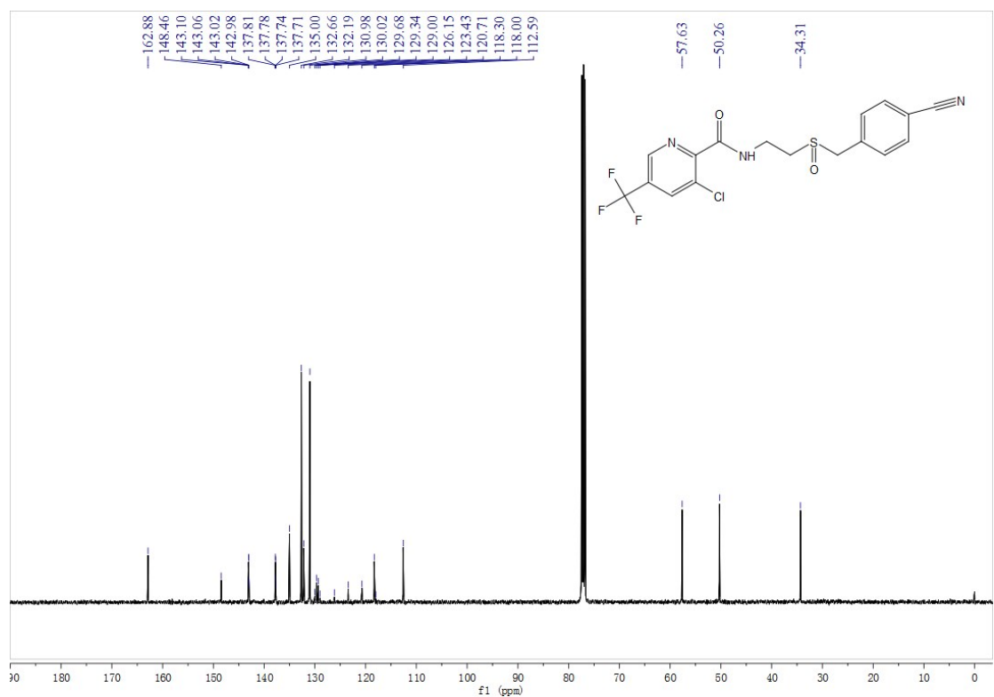
Fig. S143 13 C NMR spectra of compound G12
