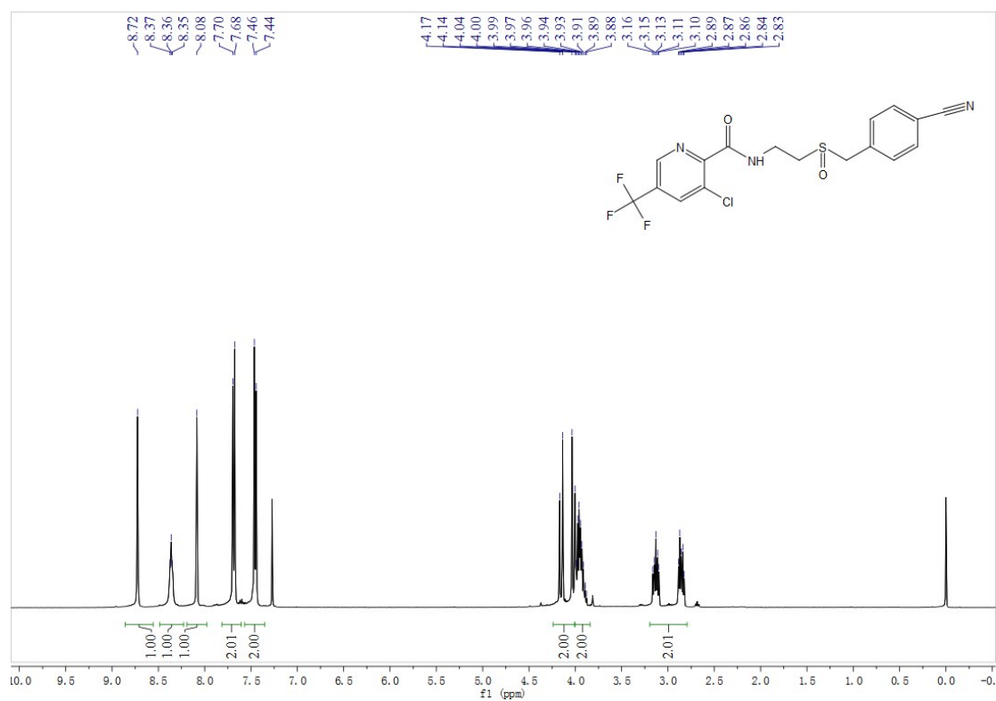
Fig. S142 1 H NMR spectra of compound G12
