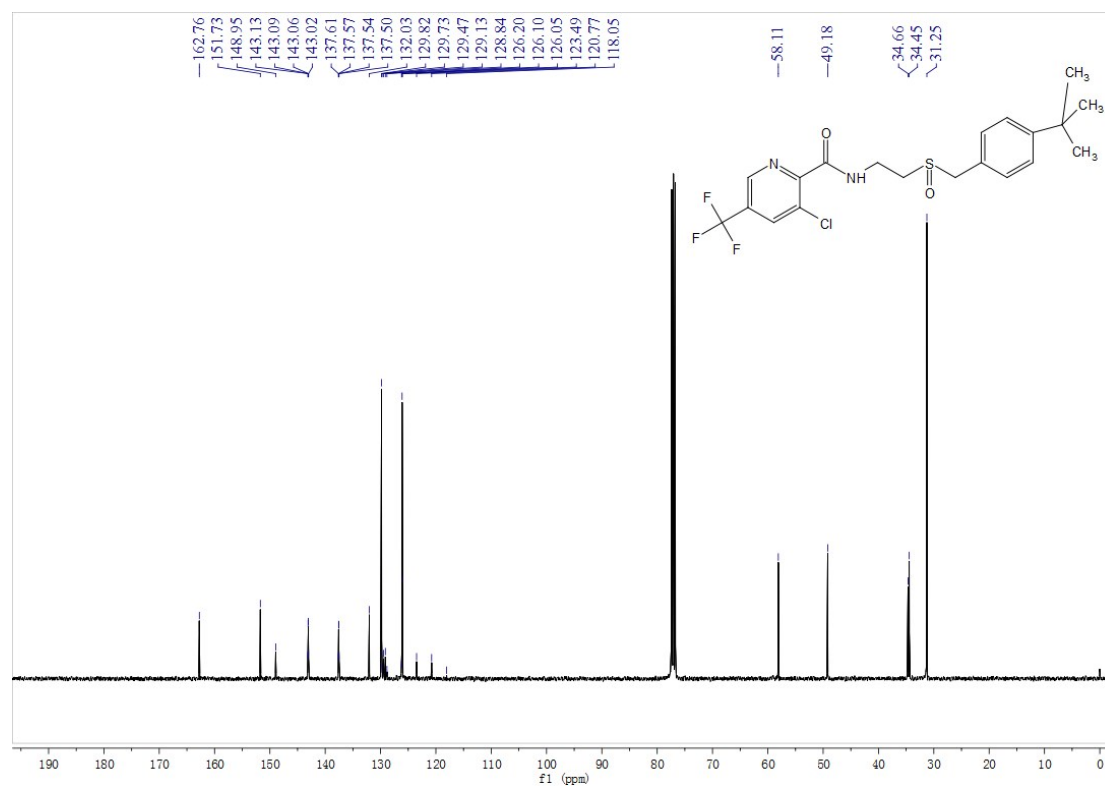
Fig. S137 13 C NMR spectra of compound G10
