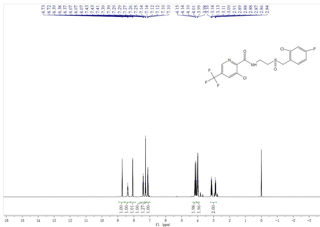
Fig. S112 1 H NMR spectra of compound G2
