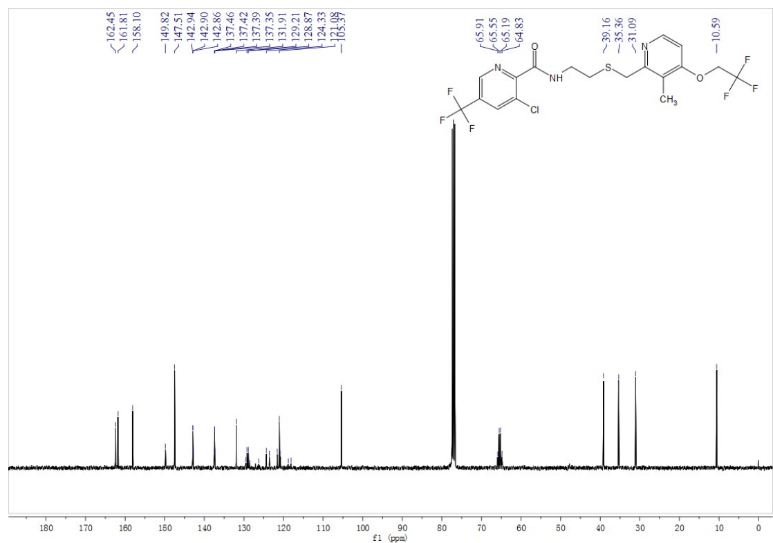
Fig. S71 13 C NMR spectra of compound E24
