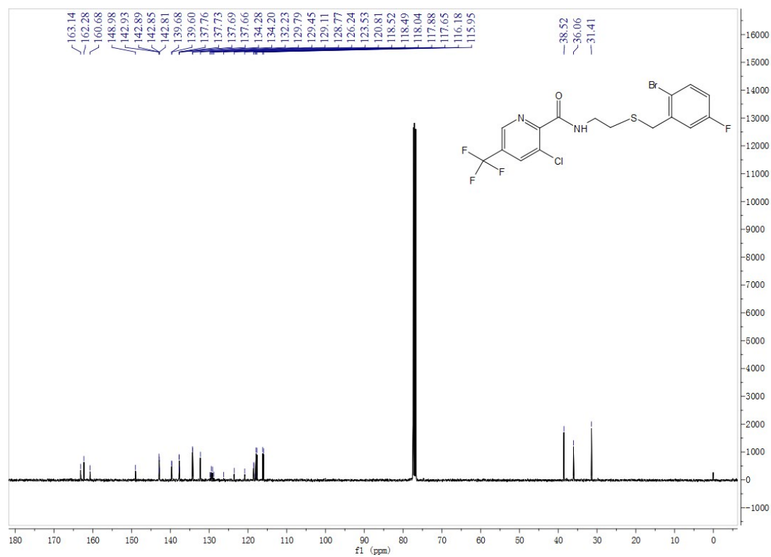
Fig. S11 13 C NMR spectra of compound E4
