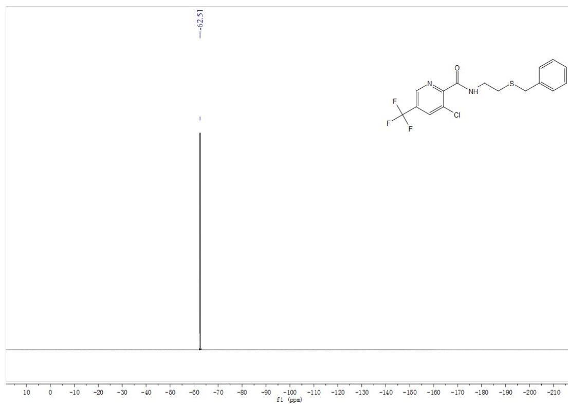
Fig. S27 ^{19}\text{F} NMR spectra of compound E9
