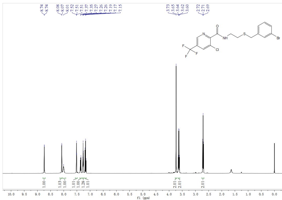
Fig. S43 1 H NMR spectra of compound E15
