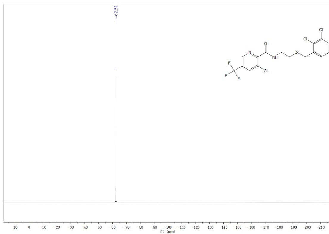
Fig. S18 ^{19}\text{F} NMR spectra of compound E6
