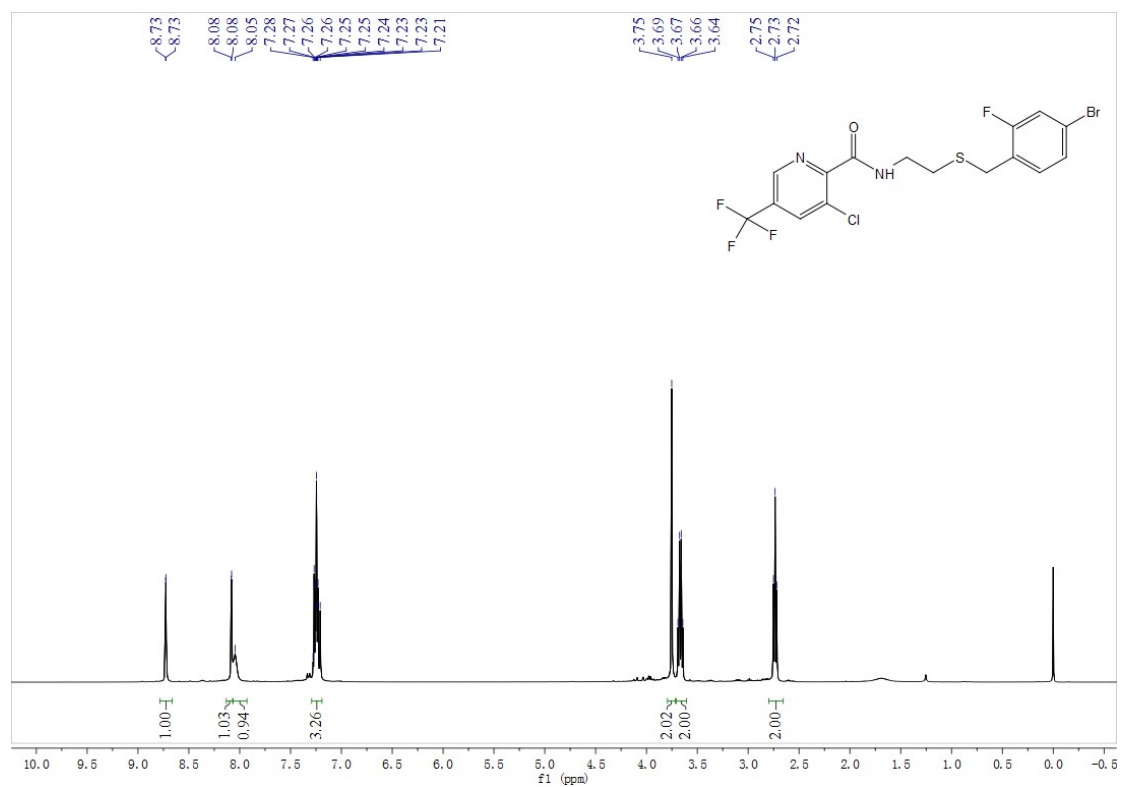
Fig. S7 1 H NMR spectra of compound E3
