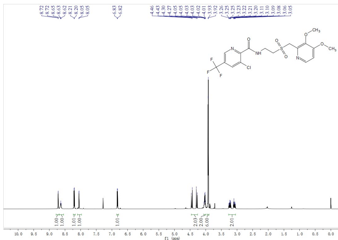
Fig. S106 1 H NMR spectra of compound F10
