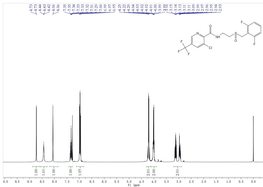
Fig. S124 1 H NMR spectra of compound G6
