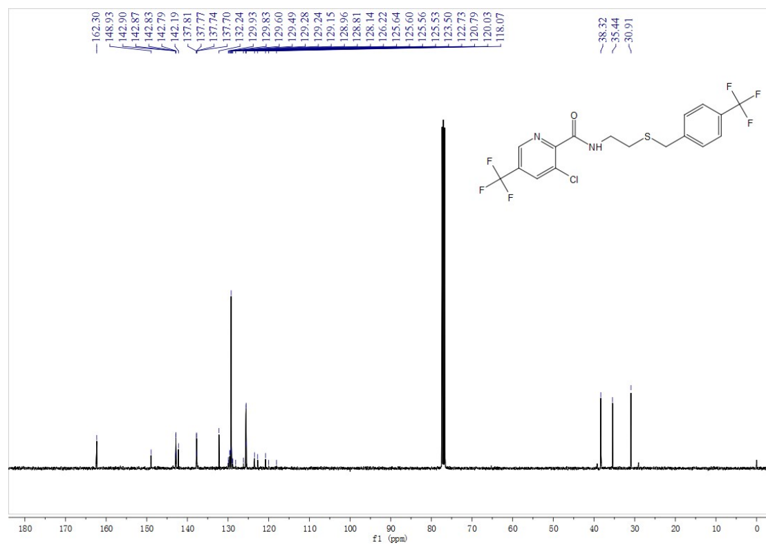
Fig. S32 13 C NMR spectra of compound E11
