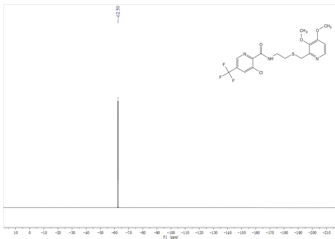
Fig. S30 ^{19}\text{F} NMR spectra of compound E10
