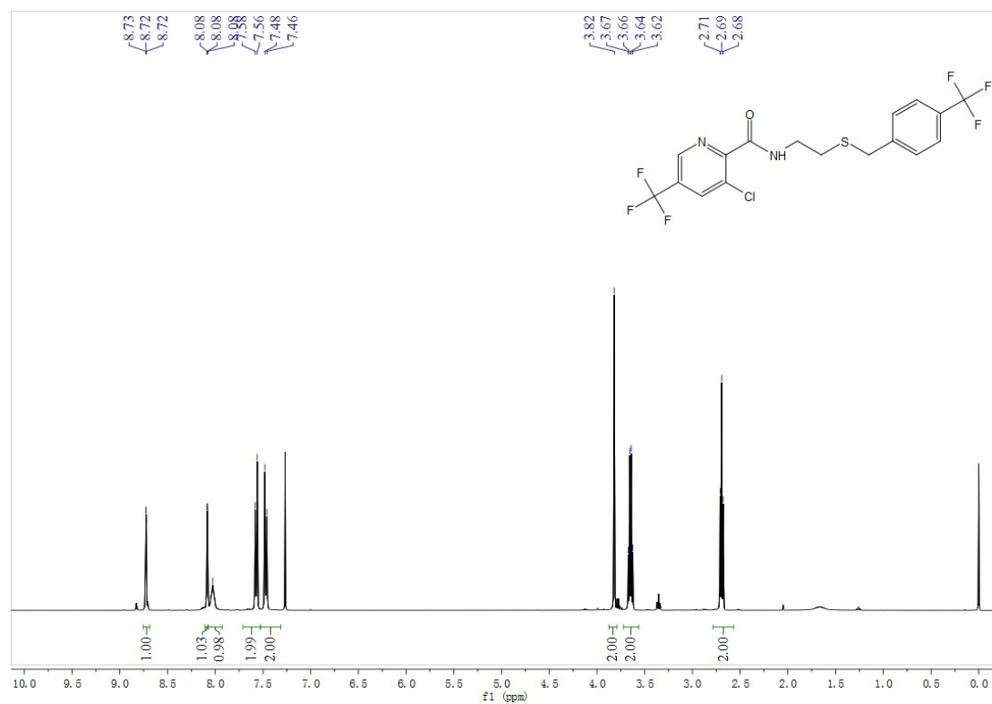
Fig. S31 1 H NMR spectra of compound E11
