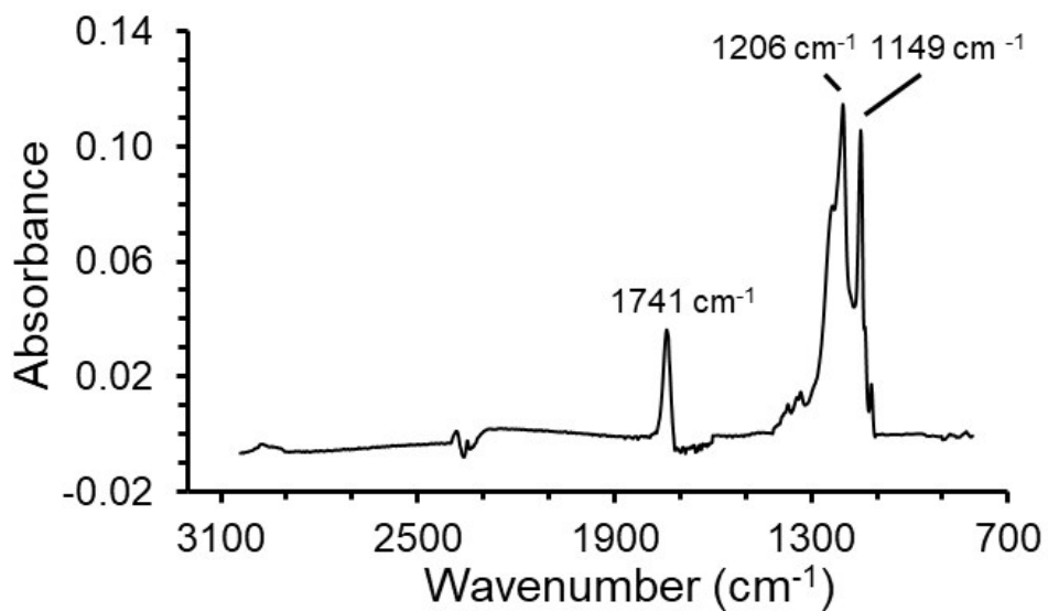
Fig. S2. FTIR spectrum of the PHDFA coating on the reference surface with deposition time of 30 min.
