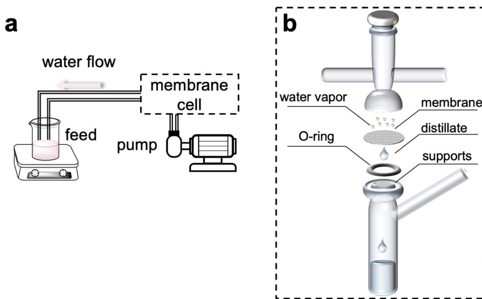
Fig. S1. Schematic illustration of (a) MD setup (b) membrane cell.
