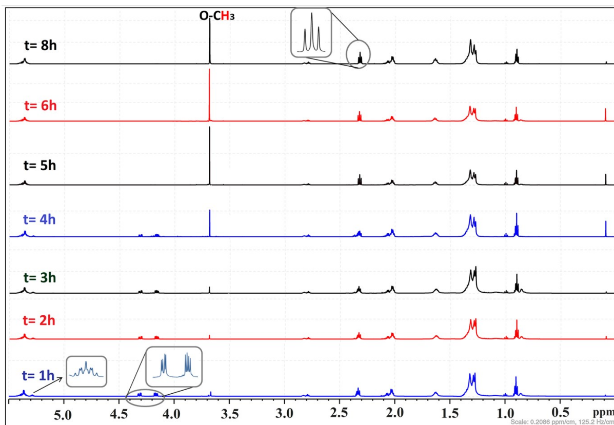
Figure S2 ^1\text{H} -NMR spectra of the biodiesel samples withdrawn at different interval of time.
