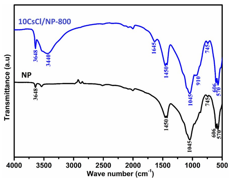
Figure S1 FTIR of NP and 10CsCl/NP-800.
