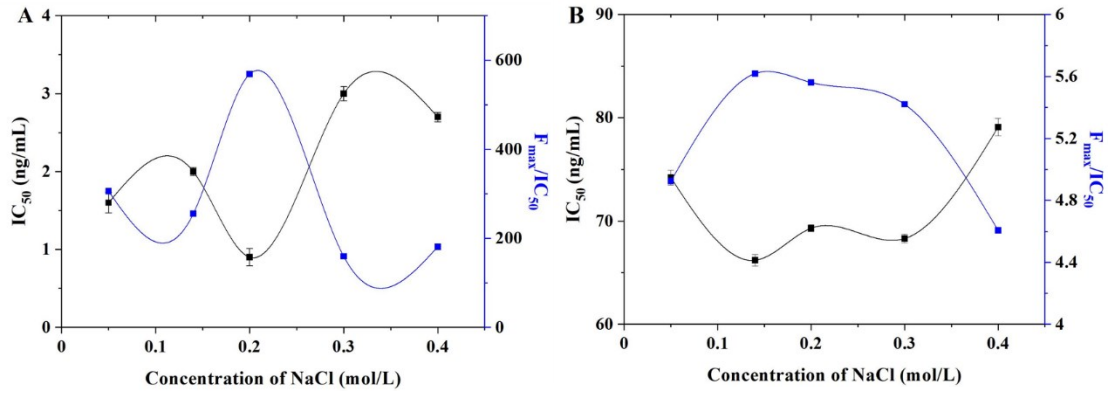
Fig. S4 Effect of concentration of NaCl on the sensitivity of the multicolor UCFIA: (A) thiamethoxam, (B) dextran 2000.
