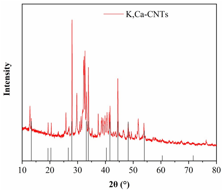
Figure S2. XRD spectra of K, Ca-CNTs.
