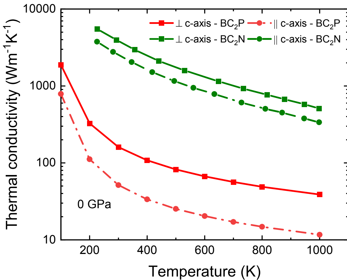
Figure S1: Thermal conductivity of hexagonal BC 2 P and BC 2 N along in-plane and out-of-plane directions at 0 GPa
