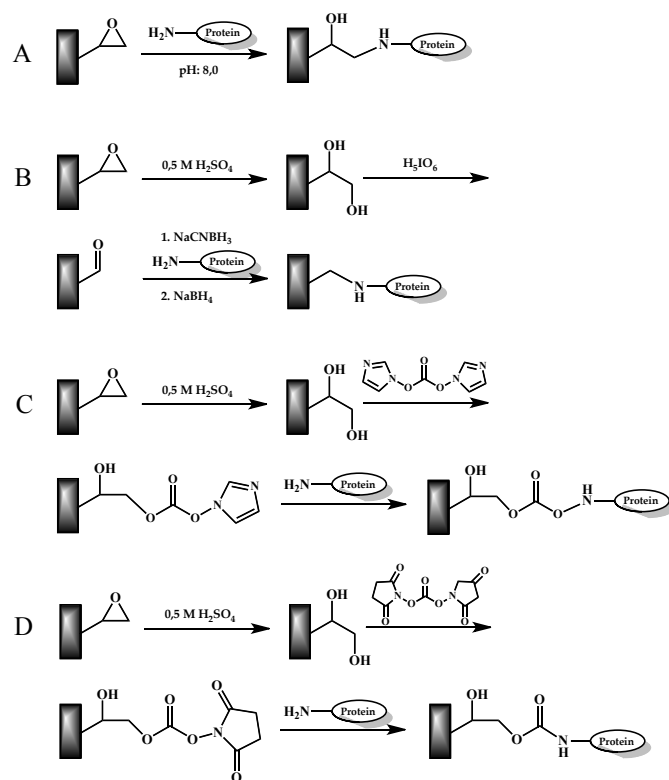
Figure 1S. Covalent immobilization of molecules with amino group, on poly (GMA-co-EDMA) monoliths. Methods of: Epoxide (A), Schiff's Base (B), Carbonyldiimidazole (C) and Disuccinimidyl (D) 33 .
