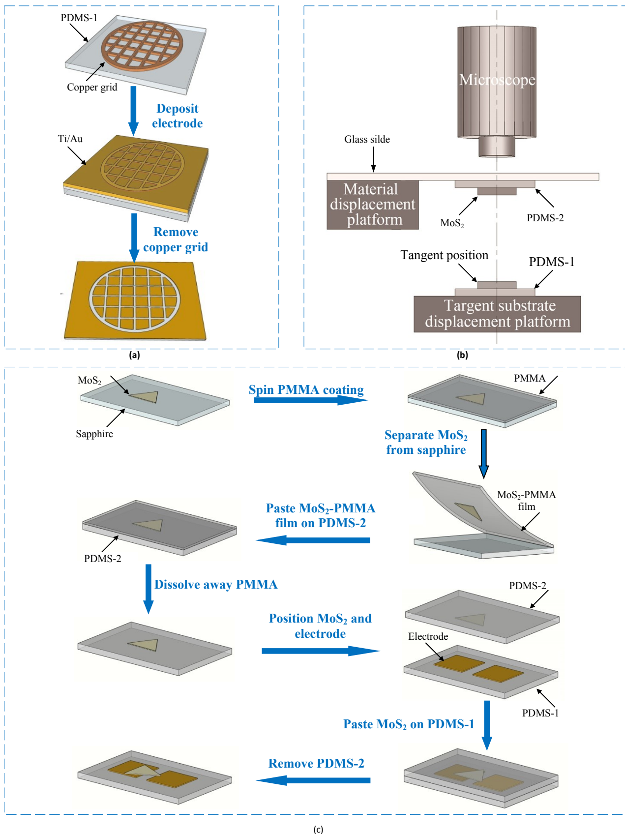
Figure S2. Operating procedures for preparation of metal electrodes on PDMS flexible substrate and transferring MoS 2 onto the flexible substrate under precise position control. a) Preparation of metal electrodes on PDMS flexible substrate. b) Schematic diagram for transfer of MoS 2 onto a flexible substrate under precise position control. c) Transfer of MoS 2 onto the flexible substrate.
