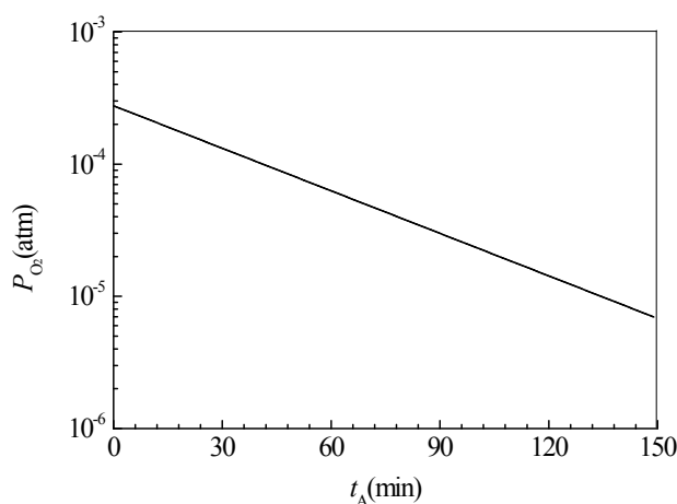
Figure S1. Dependence of the partial pressures of oxygen on the subsequent aeration time since the moment when the inert gas has been injected to 1 atm.
