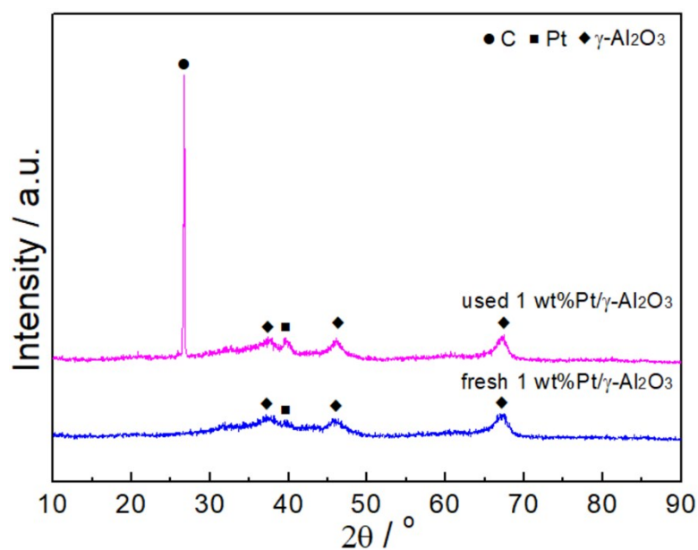
Fig. S1 XRD patterns of fresh and used Pt/ \gamma -Al 2 O 3 catalysts.
