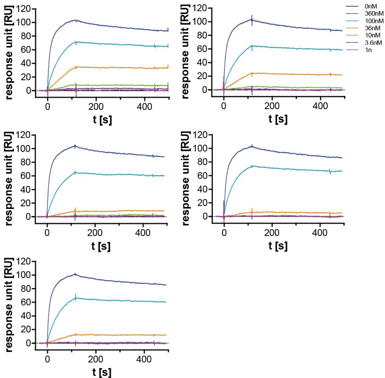
Supporting Figure 11: Surface Plasmon Resonance (SPR) measurement of clickmer B1 modified with Bn-dU in D-PBS buffer at 37°C. Streptavidin in different concentration was used as analyte and clickmer was used as an immobilized ligand ( n=5 ).
