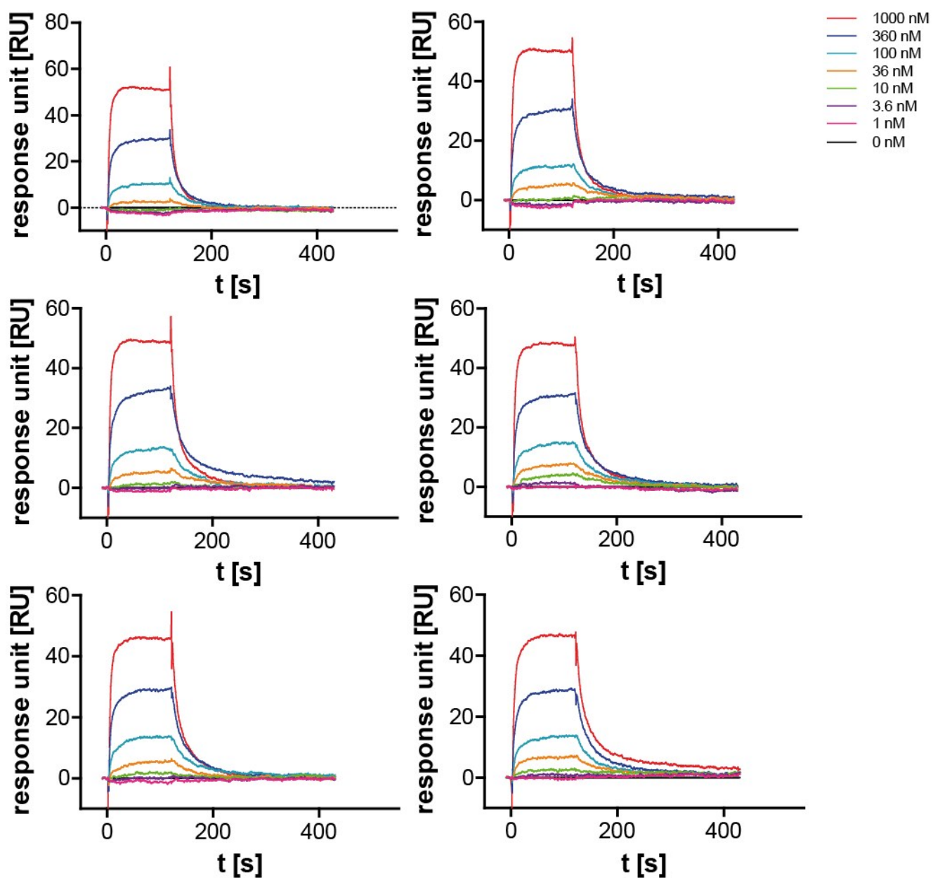
Supporting Figure 9: Surface Plasmon Resonance (SPR) measurement of clickmer B33 modified with Bn-dU at 37°C. C3-GFP in different concentration was used as analyte and clickmer was used as an immobilized ligand ( n=6 ).
