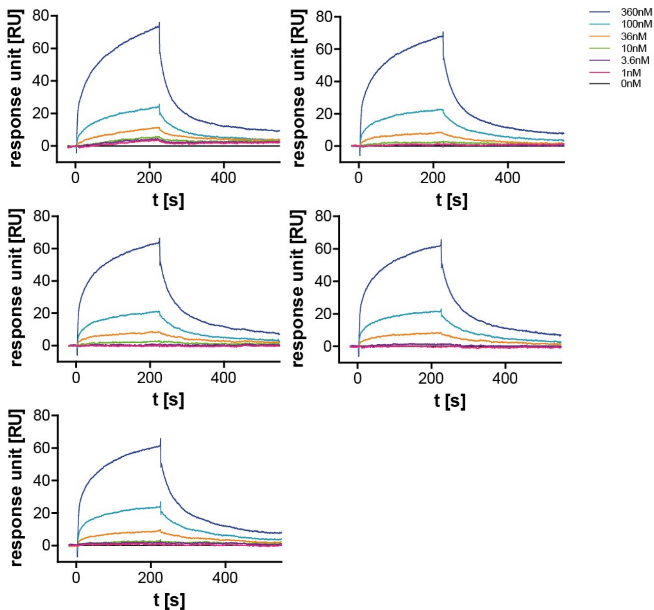
Supporting Figure 8: Surface Plasmon Resonance (SPR) measurement of clickmer B33 modified with Bn-dU at 25°C. C3-GFP in different concentration was used as analyte and clickmer was used as an immobilized ligand ( n=5 ).
