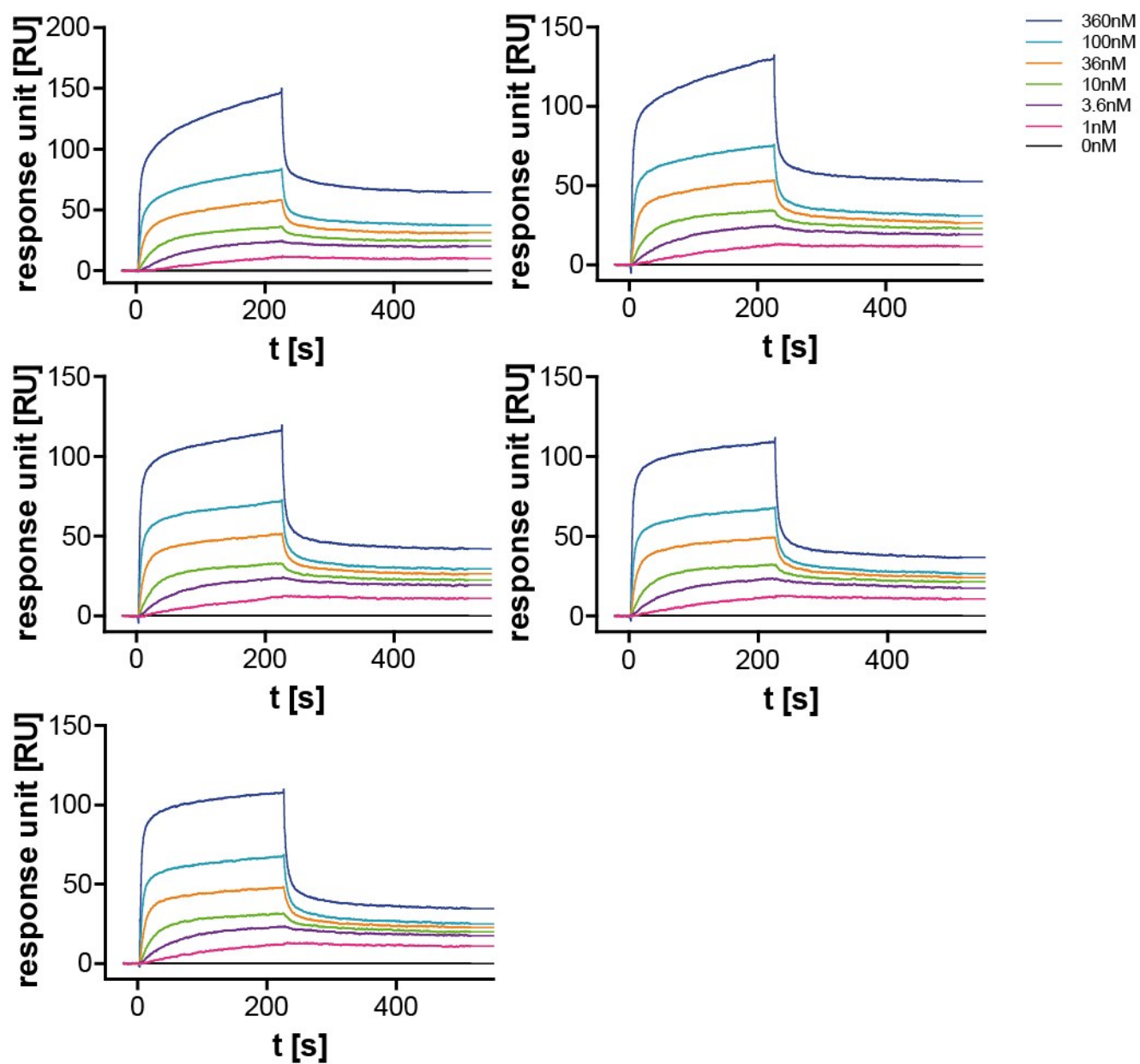
Supporting Figure 6: Surface Plasmon Resonance (SPR) measurement of clickmer F20 modified with BF-dU at 25°C. C3-GFP in different concentration was used as analyte and clickmer was used as an immobilized ligand (n=5).
