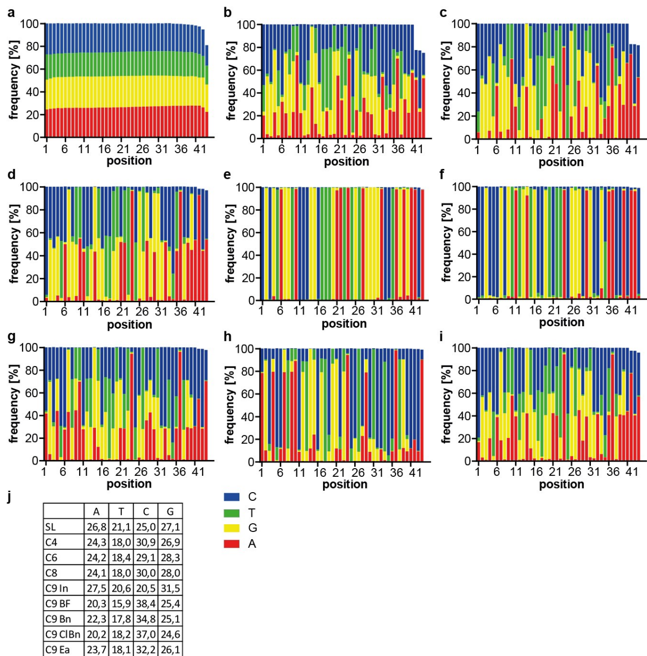
Supporting Figure 2: NGS analysis of all selection cycles of the split-combine SELEX targeting C3-GFP. Statistical base distribution over the 44 nucleobases random region for the starting library (a), selection cycle 4 (b), cycle 6 (c), cycle 8 (d), and cycle 9 for indole azide (In-dU) (e), cycle 9 for benzofuran azide (BF-dU) (f), and cycle 9 for benzyl azide (Bn-dU) (g), cycle 9 for chlorobenzyl azide (ClBn-dU) (h), and cycle 9 for amine azide (Ea-dU) (i). (j) Shown is the distribution of the nt in the random region [%].
