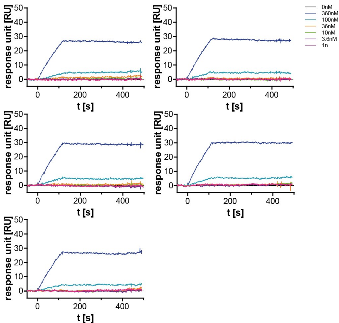
Supporting Figure 13: Surface Plasmon Resonance (SPR) measurement of aptamer G1 (naïve, unmodified DNA) in D-PBS buffer at 21°C. Streptavidin in different concentration was used as analyte and clickmer was used as an immobilized ligand ( n=5 ).
