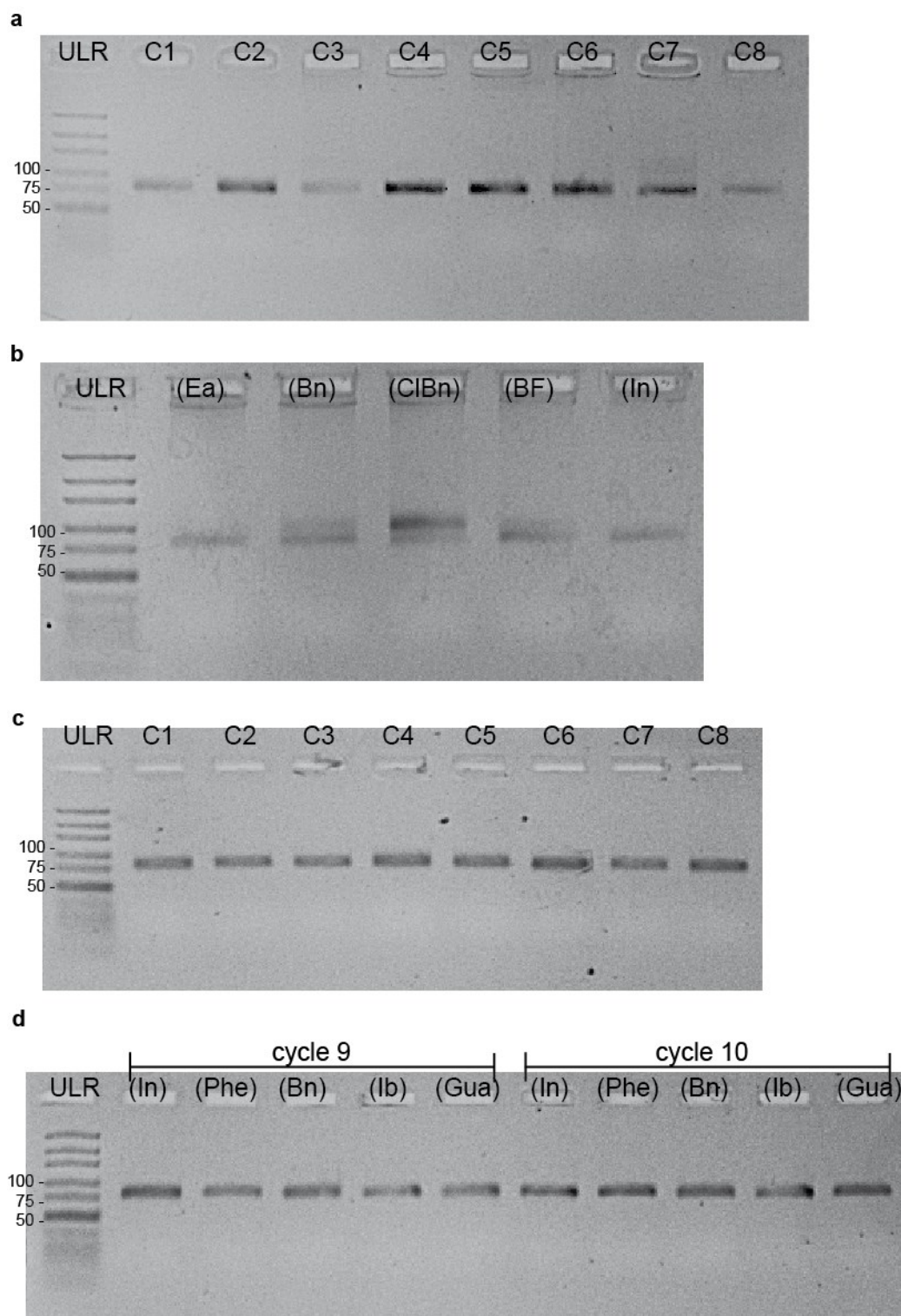
Supporting Figure 1: Agarose gel electrophoresis analysis of the PCR products from split-combine SELEX. In (a) the first eight selections cycles targeting C3-GFP and in (b) the ninth cycle with the different azides ((In) 3-(2-azidoethyl)-1 H -indole, (BF) 3-(2-azidoethyl)-benzofuran, (ClBn) 1-(azidomethyl)-4-chlorobenzene, (Bn) 1-(azidomethyl)-benzene, and (Ea) 2-azidoethanamine) are depicted. For this SELEX the OW1 library was used (dsDNA: 80 bp). In (c) the first eight selections cycles targeting SA and in (d)
