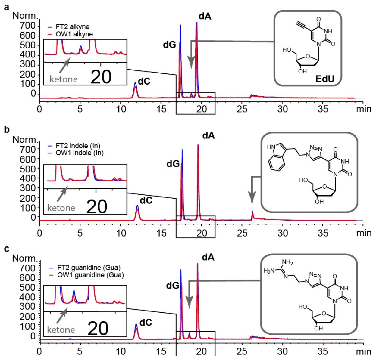
HPLC analysis of the libraries FT2 and OW1. The non-functionalized DNA (alkyne) (a), the indole (In) (b), and guanidine (Gua) (c) modified libraries were digested to the nucleotide level and analysed by HPLC.
