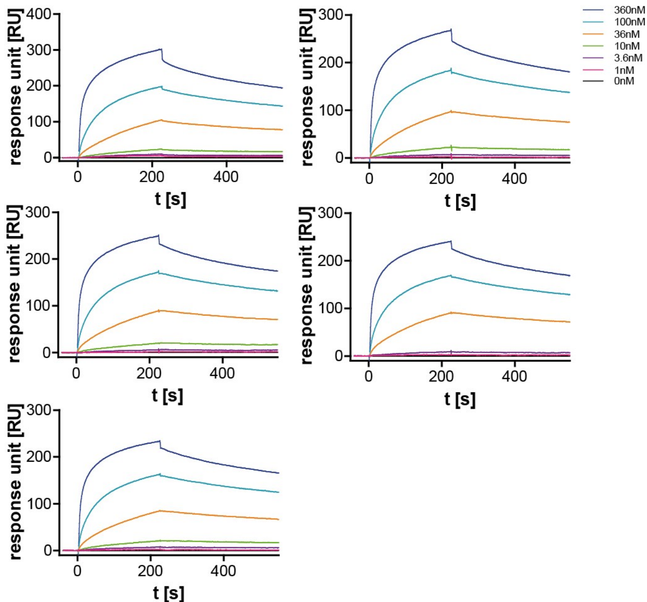
Supporting Figure 4: Surface Plasmon Resonance (SPR) measurement of clickmer I10 modified with In-dU at 25°C. C3-GFP in different concentration was used as analyte and clickmer was used as an immobilized ligand (n=5).
