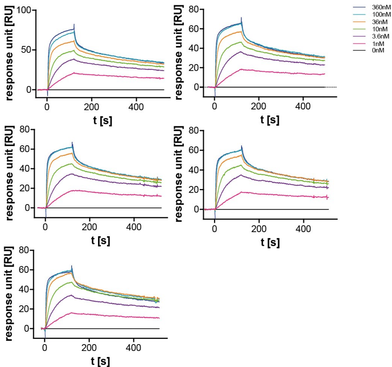
Supporting Figure 7: Surface Plasmon Resonance (SPR) measurement of clickmer F20 modified with BF-dU at 37°C. C3-GFP in different concentration was used as analyte and clickmer was used as an immobilized ligand (n=5).
