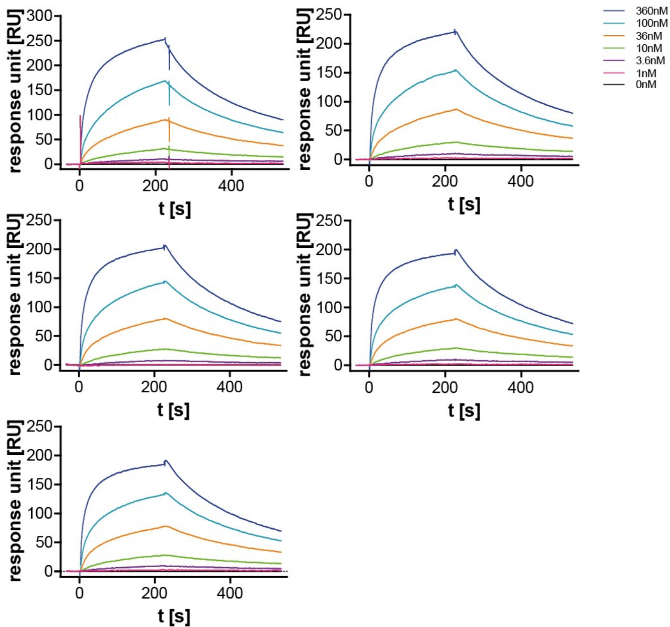
Supporting Figure 5: Surface Plasmon Resonance (SPR) measurement of clickmer I10 modified with In-dU at 37°C. C3-GFP in different concentration was used as analyte and clickmer was used as an immobilized ligand ( n=5 ).
