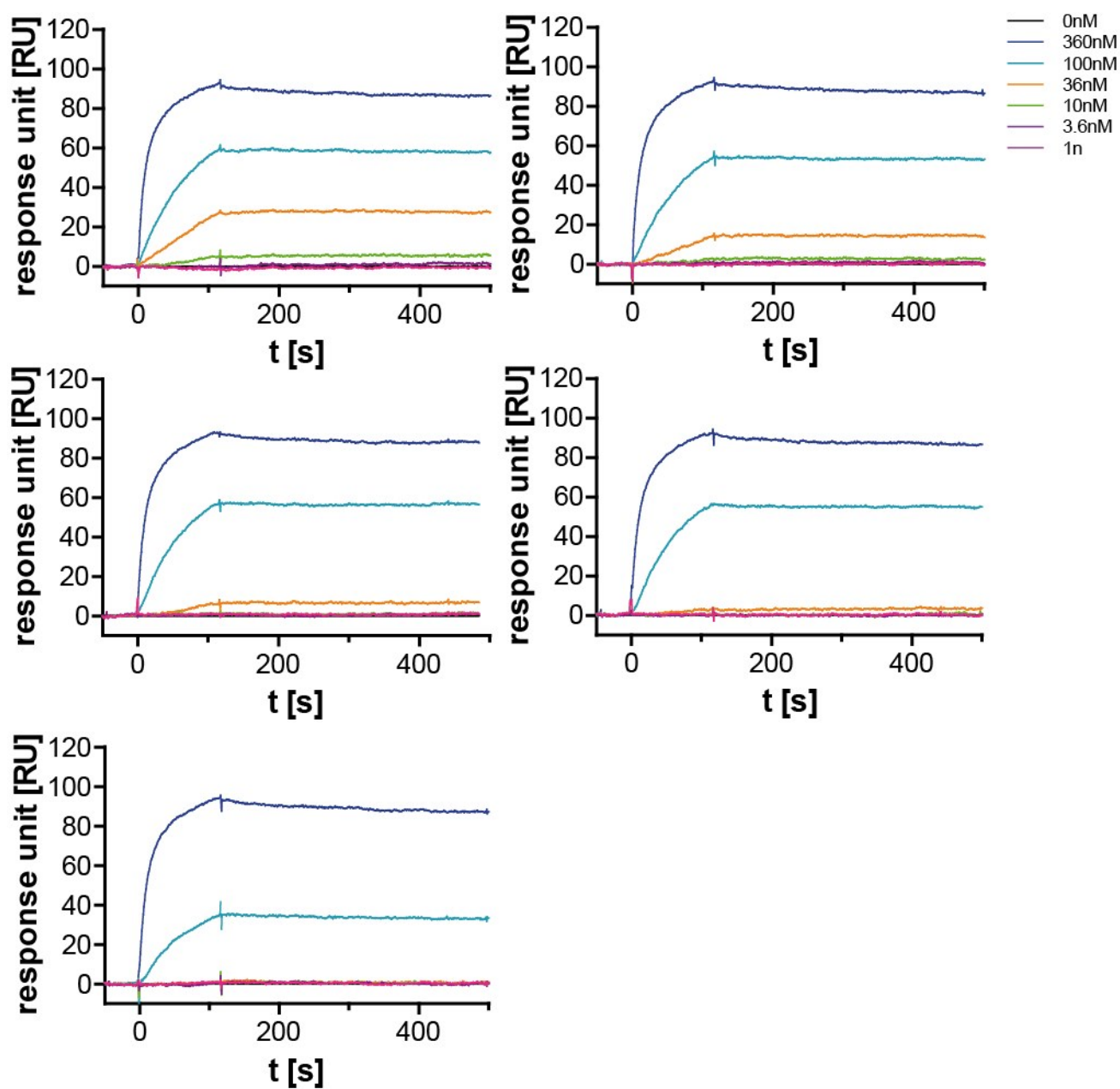
Supporting Figure 12: Surface Plasmon Resonance (SPR) measurement of clickmer B1 modified with Bn-dU in D-PBS buffer at 21°C. Streptavidin in different concentration was used as analyte and clickmer was used as an immobilized ligand (n=5).
