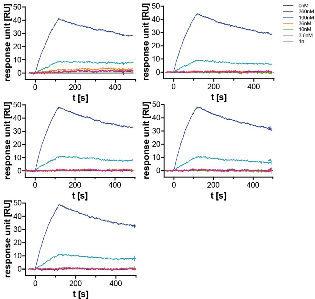
Supporting Figure 14: Surface Plasmon Resonance (SPR) measurement of aptamer G1 (naïve, unmodified DNA) in D-PBS buffer at 37°C. Streptavidin in different concentration was used as analyte and clickmer was used as an immobilized ligand (n=5).
