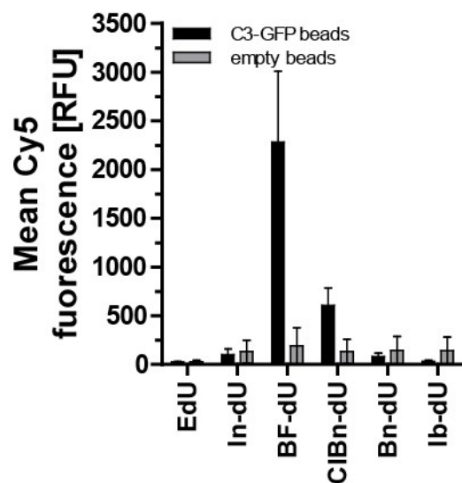
Supporting Figure 3: Flow cytometer binding assay in which 500 nM Cy-5 labelled DNA from the clickmer C1 were incubated with C3-GFP immobilized on magnetic beads (C3-GFP beads). DNA was unmodified (Edu) or modified with indole (In-dU), benzofuran (BF-dU), benzyl (Bn-dU), chlorobenzyl (ClBn-dU) or isobutyl (Ib-dU) (experiments were done at least twice in duplicates, mean \pm SD).
