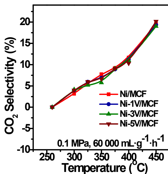
Fig. S2 CO 2 selectivity of the different catalysts.
