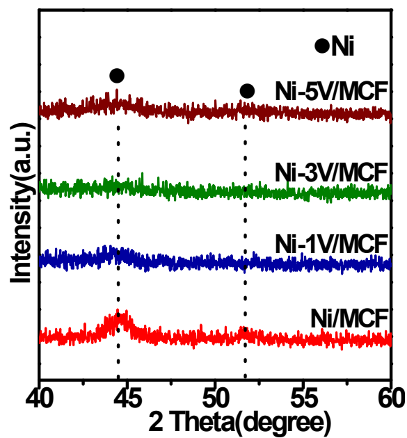
Fig. S1 XRD patterns of the reduced catalysts.
