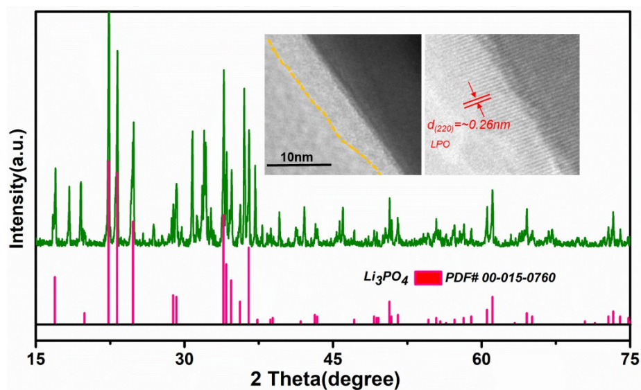
Figure S1. The XRD patterns of additional experimental product; and HRTEM image of coating layer.
