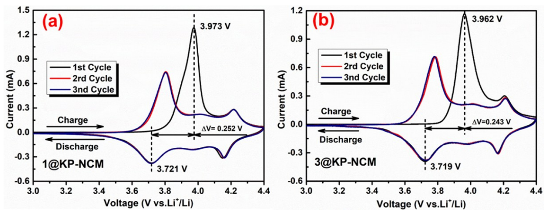
Figure S2. The CV curves of 1@KP-NCM (a) and 3@KP-NCM (b) tested between 3.0 and 4.4V at 0.1 mV s -1 .
