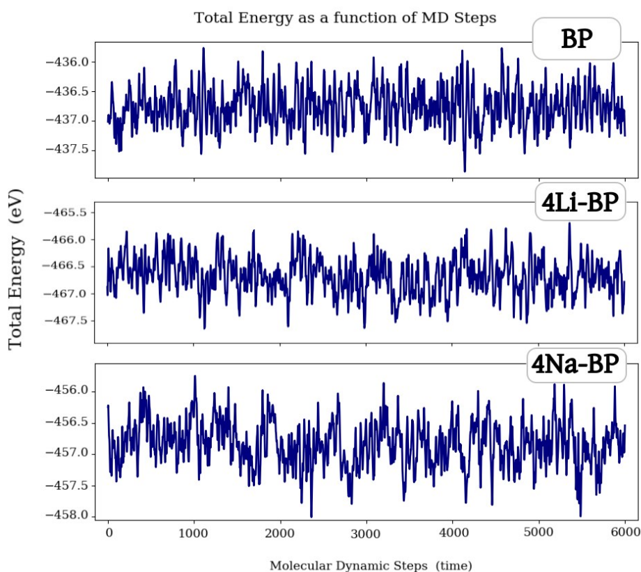
Figure S2. Thermal stability of 2D BP, 4Li@BP and 4Na@BP monolayers, the variation of the total-energy between 0 and 6 ps during the ab-initio molecular dynamics (AIMD) simulations at room temperature.
