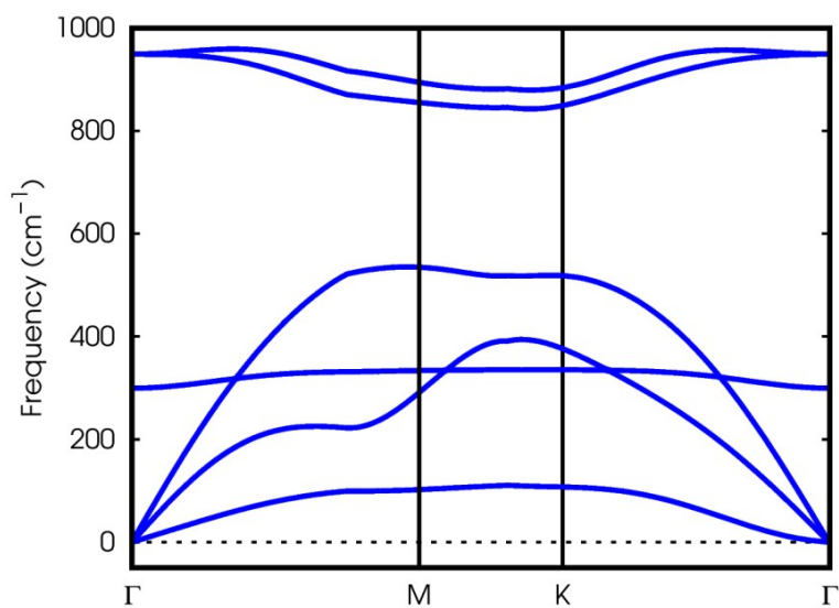
Figure S1. Dynamical stability of 2D BP monolayer, the phonon dispersion pattern along the k-vectors with high symmetry.
