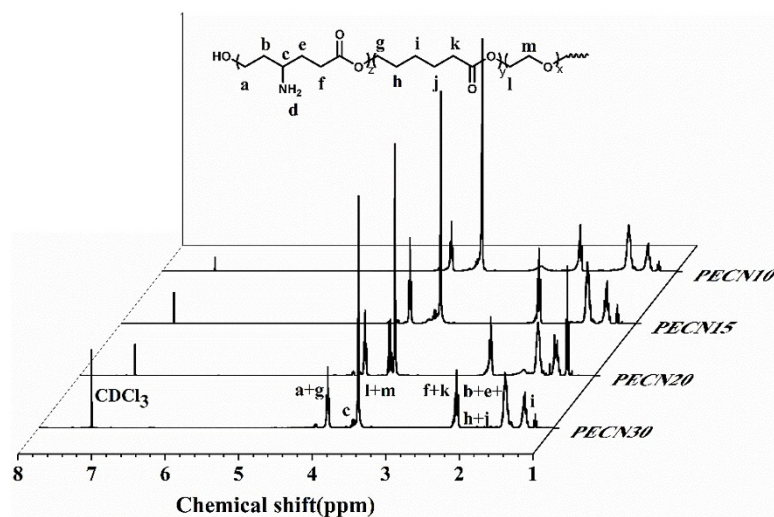
Fig. S3. ^1\text{H} NMR spectra of PECN10, PECN15, PECN20 and PECN30
