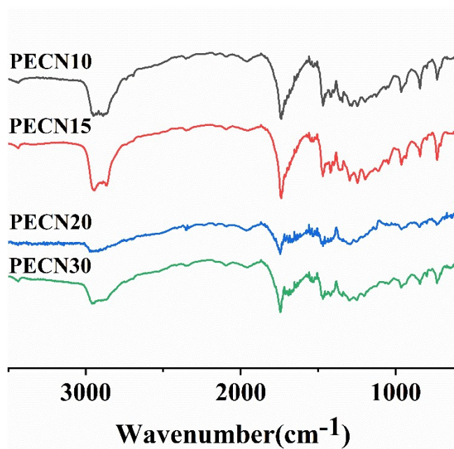
Fig. S4. FT-IR spectra of PECN10, PECN15, PECN20, PECN30
