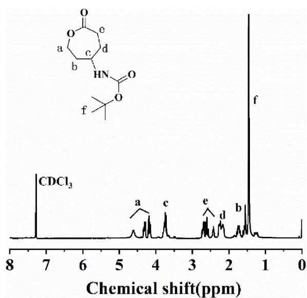
Fig. S2. 1 H NMR spectra of Boc-NCL
