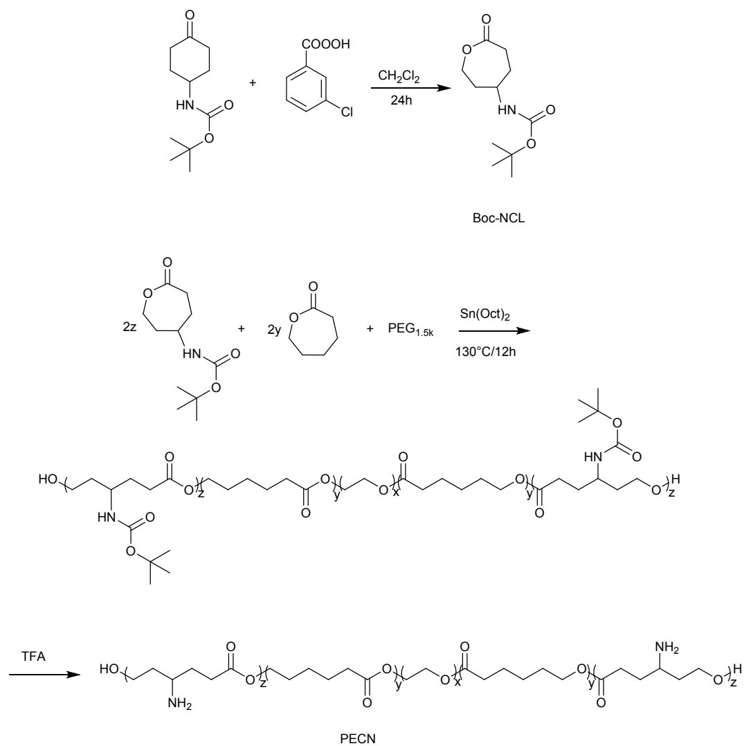
Fig. S1. Synthetic route of PECN
