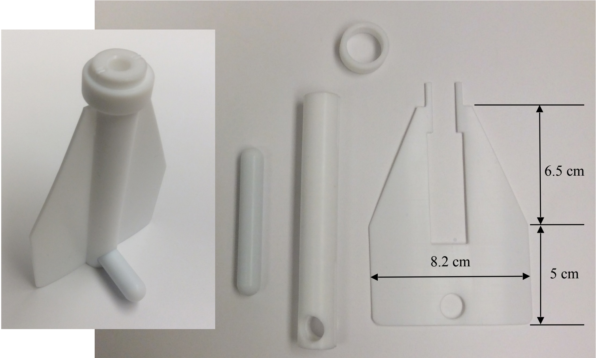
"stretch" impeller design
