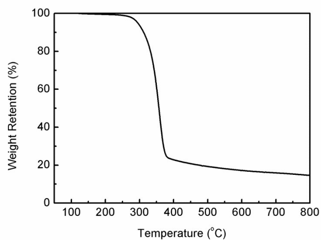
Fig. S3. TGA curve of golf ball-like SiO 2 -SH particles.
