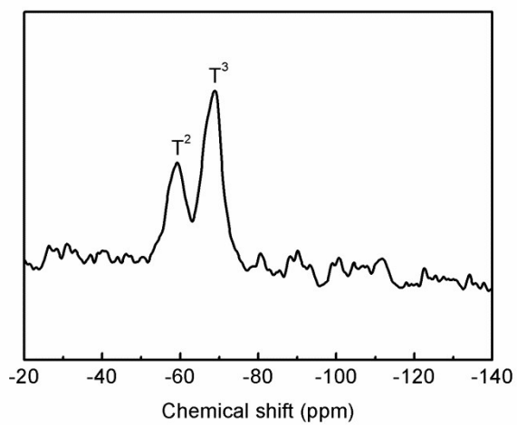
Fig. S4. Solid state 29 Si NMR spectrum of the golf ball-like SiO 2 -SH particles.
