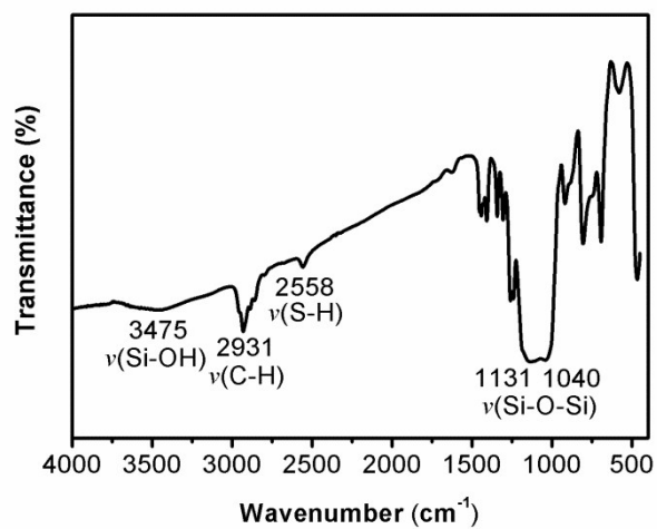
Fig. S1. FT-IR spectrum of the golf ball-like SiO 2 -SH particles.
