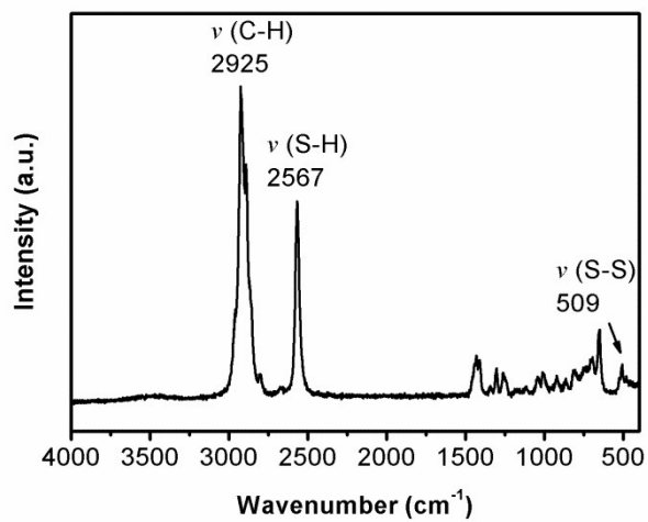
Fig. S2. Raman spectrum of the golf ball-like SiO 2 -SH particles.
