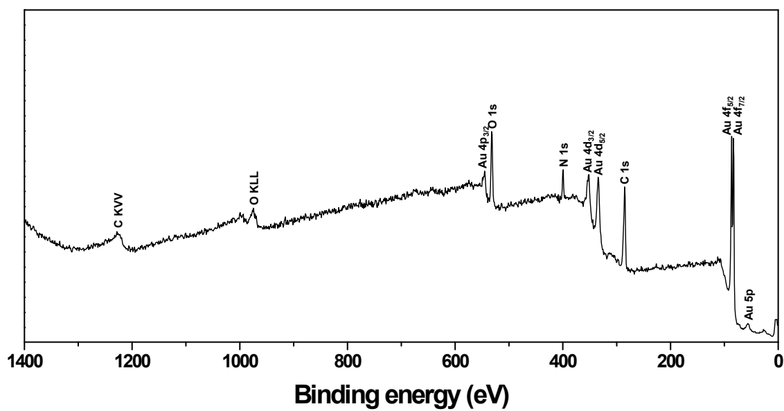
Figure S3: XPS survey spectrum of AuNPs-SS.
