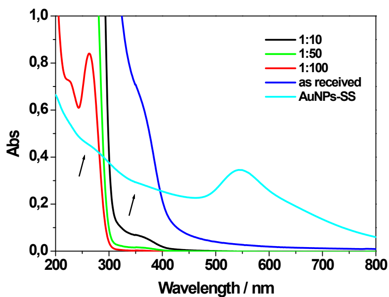
Figure S1: A comparison between the UV-Vis spectra of SS solutions performed at different dilutions and AuNPs-SS.
