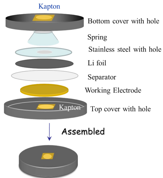
Figure S1: Schematic drawing of perforated coin cell assembly used for TXM analysis.
