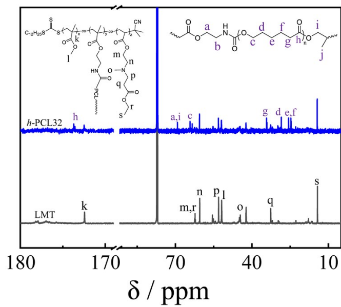
Figure S3. ^{13}\text{C} NMR spectra of LMT and h -PCL32 in \text{CDCl}_3 .
