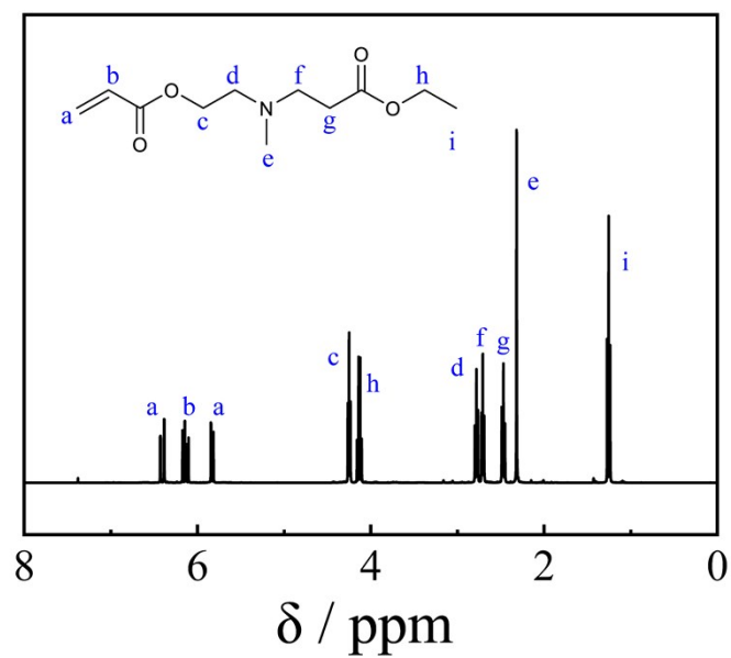
Figure S1. 1 H NMR spectrum of TCB in CDCl 3 .
