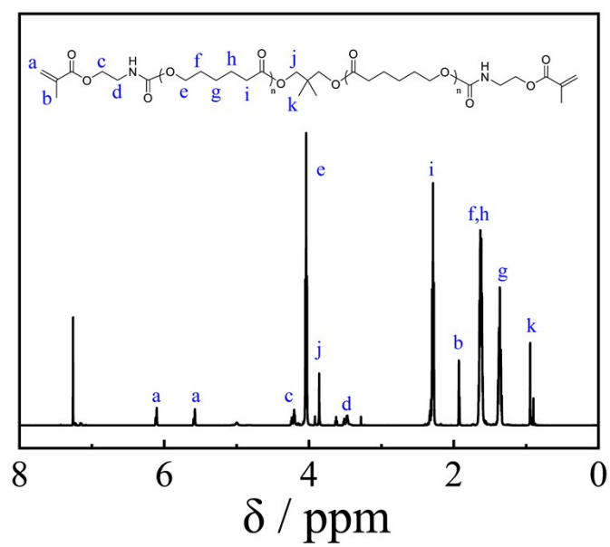
Figure S2. 1 H NMR spectrum of PCL-V 2 in CDCl 3 .
