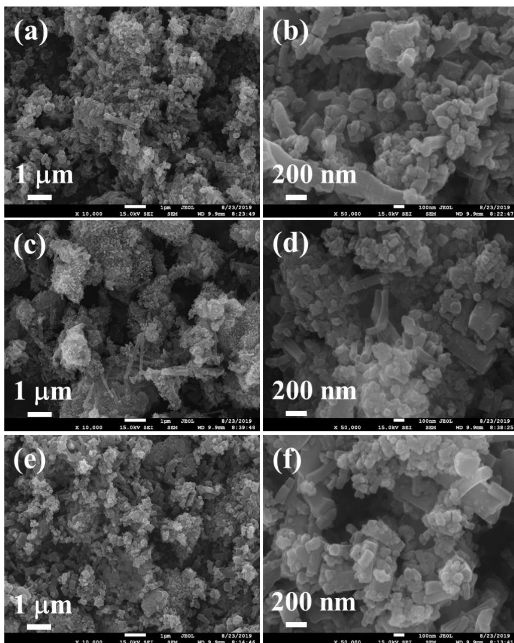
Fig. S4 Low- and high-magnification SEM images of the (a, b) \text{Cu}_3(\text{HHTP})_2 , (c, d) \text{Ni}_3(\text{HHTP})_2 , and (e, f) \text{Cu}_x\text{Ni}_{3-x}(\text{HHTP})_2 MOFs.
