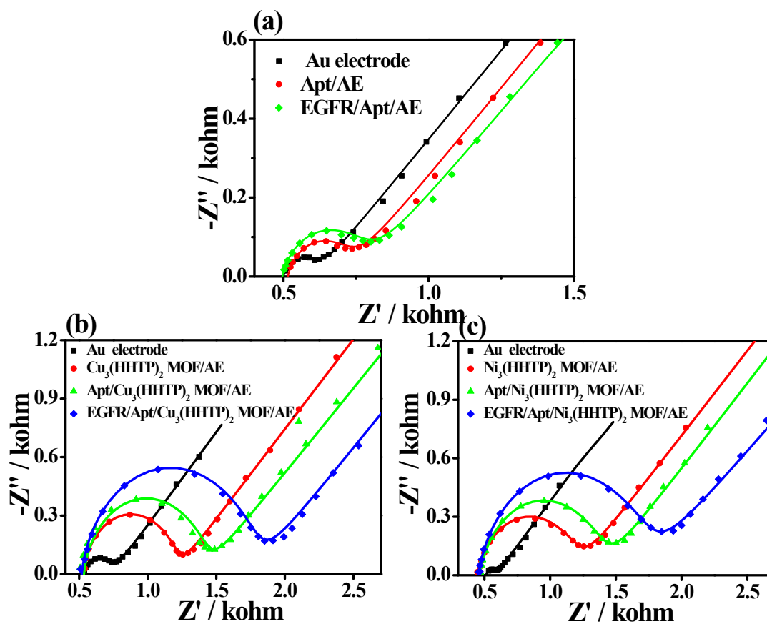
Fig. S12 EIS Nyquist plots of the aptasensors based on of (a) the bare Au electrode, (b) \text{Cu}_3(\text{HHTP})_2 , and (c) \text{Ni}_3(\text{HHTP})_2 MOFs for detecting EGFR ( 1 \text{ pg} \cdot \text{mL}^{-1} ) in PBS containing 5.0 \text{ mM } [\text{Fe}(\text{CN})_6]^{3-/4-} .
