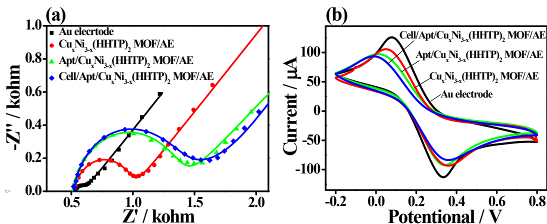
Fig. S9 (a) EIS Nyquist plots and (b) corresponding CV curves for the \text{Cu}_x\text{Ni}_{3-x}(\text{HHTP})_2 \text{ MOF} -based aptasensor for detecting L929 cells ( 1 \times 10^5 \text{ cell mL}^{-1} ) in PBS containing 5.0 \text{ mM } [\text{Fe}(\text{CN})_6]^{3-/4-} .
