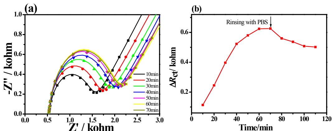
Fig. S13 (a) EIS Nyquist plots of the \text{Cu}_x\text{Ni}_{3-x}(\text{HHTP})_2 MOF-based aptasensor incubated with EGFR ( 1 \text{ pg} \cdot \text{mL}^{-1} ) for different durations and (b) their corresponding \Delta R_{ct} values.
