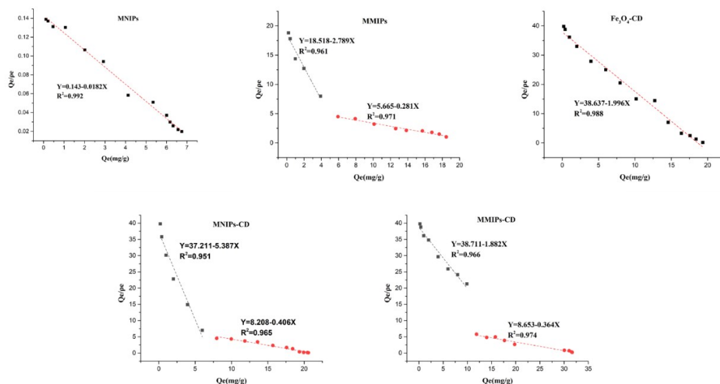
Figure S1. Static adsorption Scatchard fitting curve (MNIPs, MMIPs, \text{Fe}_3\text{O}_4\text{-CD} , MNIPs-CD, MMIPs-CD)
