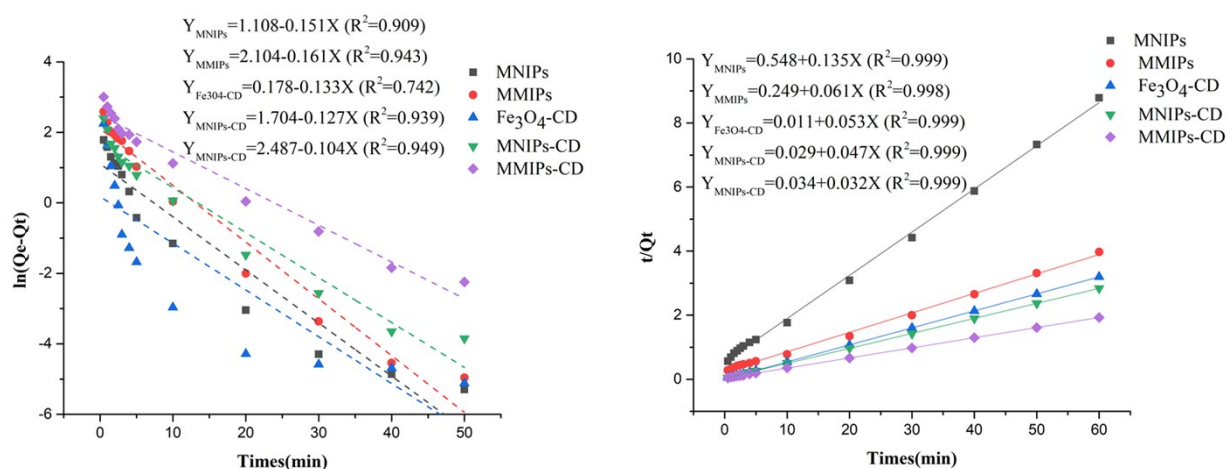
Figure S3. Dynamic adsorption fitting curve (A. pseudo-first-order plot B. pseudo-second-order plot)
