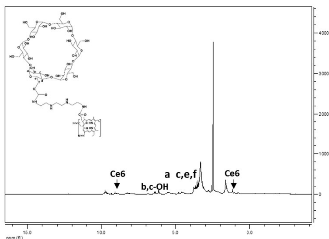
Fig S3. 1 H NMR spectra of the synthesis process of α-CD-Ce6.
