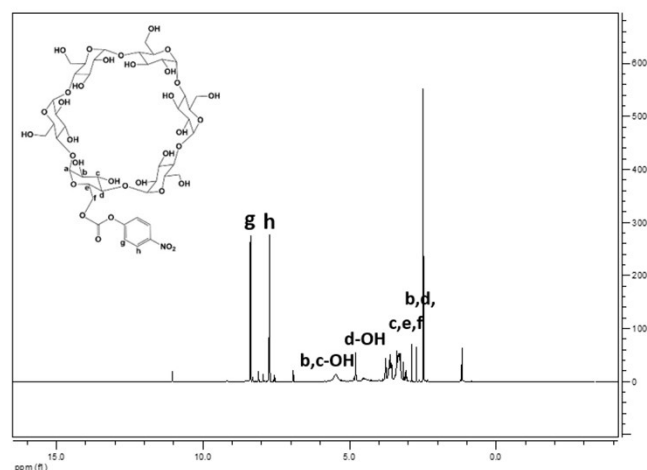
Fig S1. 1 H-NMR spectra of the synthesis process of α-CD-NC.
