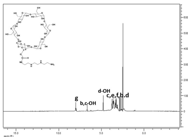
Fig S2. 1 H-NMR spectra of the synthesis process of α-CD-NH 2 .
