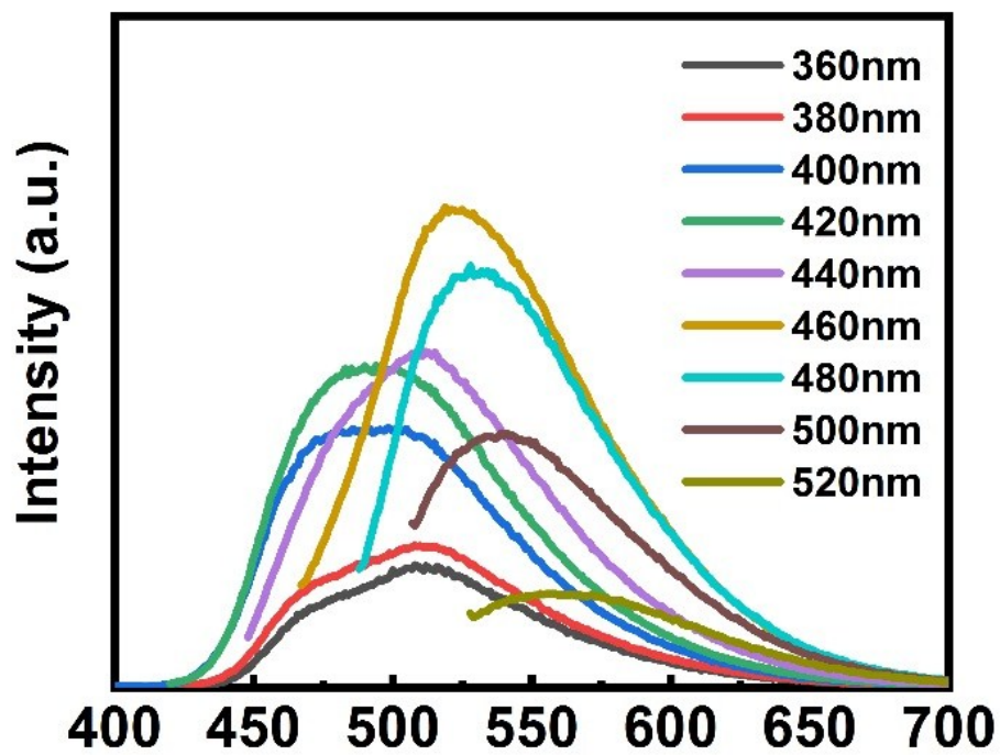
Figure S4. PL emission spectra of the G-CDs under different excitation wavelengths.
