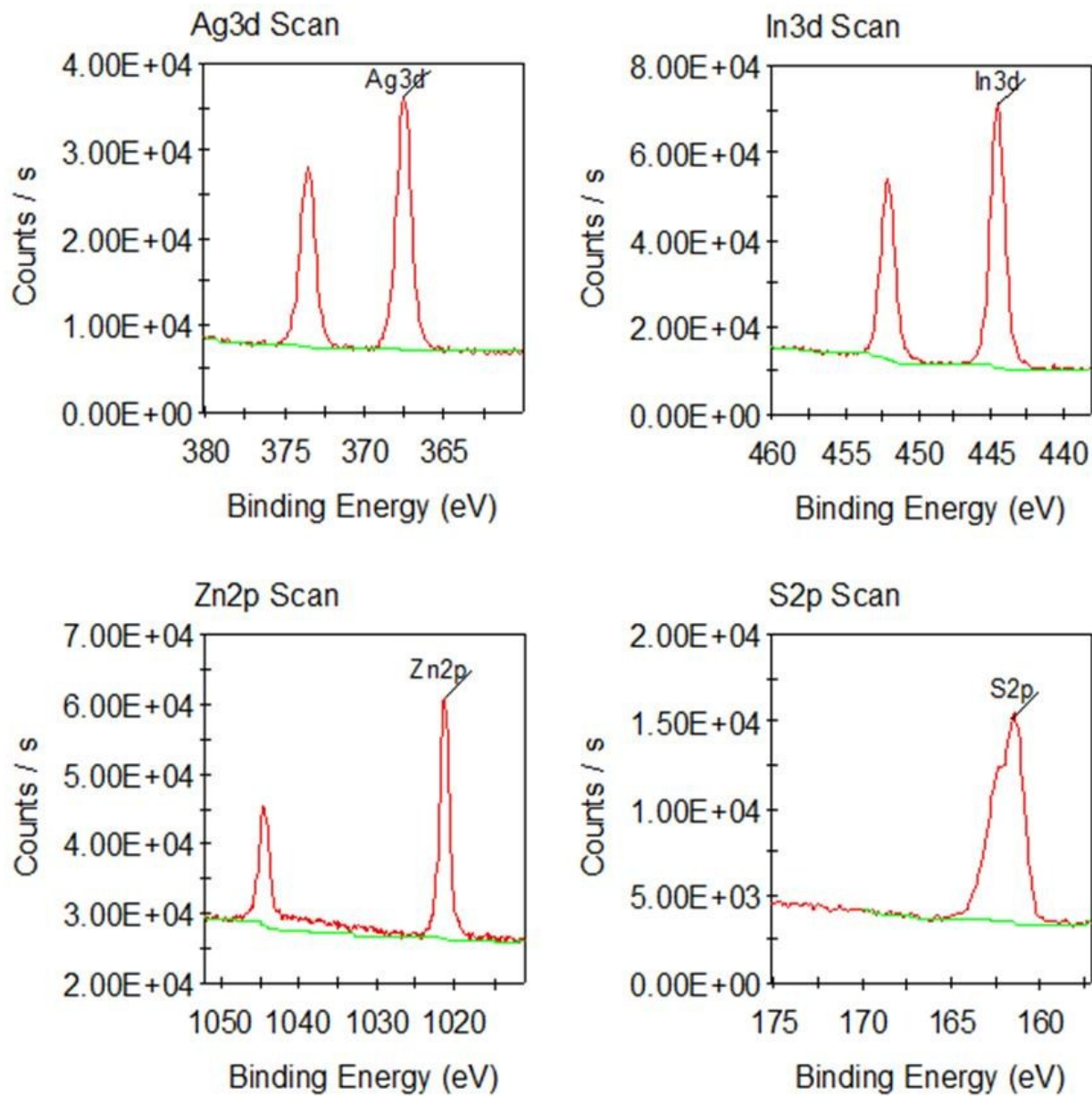
Figure S1. High-resolution XPS pattern of AIZS.
