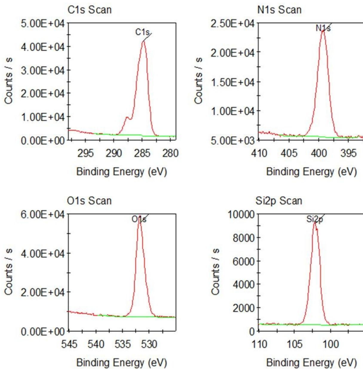
Figure S3. High-resolution XPS pattern of G-CDs
