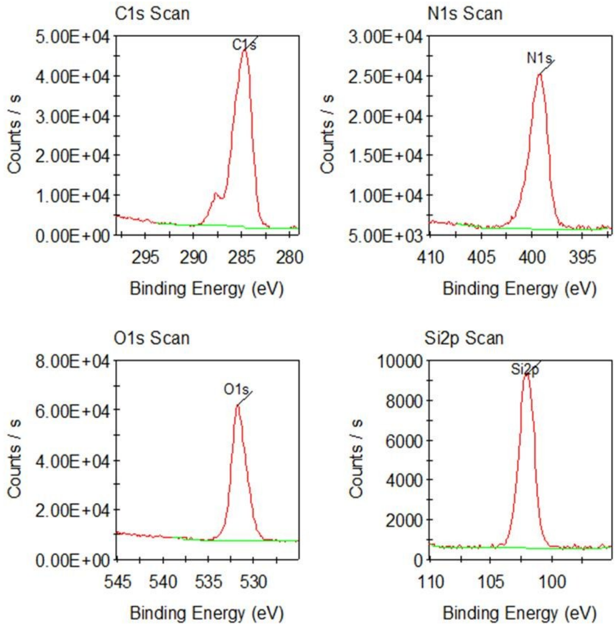
Figure S2. High-resolution XPS pattern of B-CDs.
