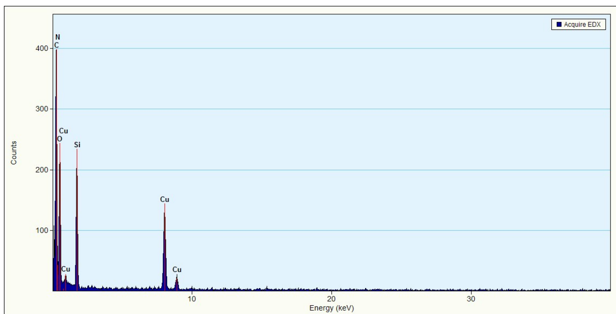
Figure S5. Energy dispersive X-ray (EDX) of CDs@SiO 2 .
