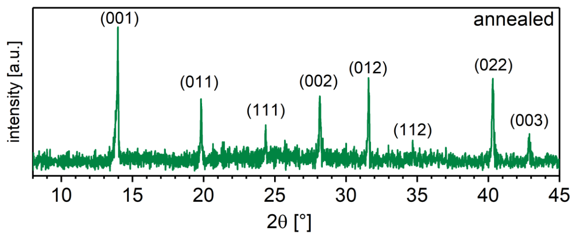
Figure S1: X-ray diffraction pattern of an annealed solution-processed \text{Cs}_{0.1}\text{FA}_{0.9}\text{PbI}_{2.9}\text{Br}_{0.1} perovskite film.
