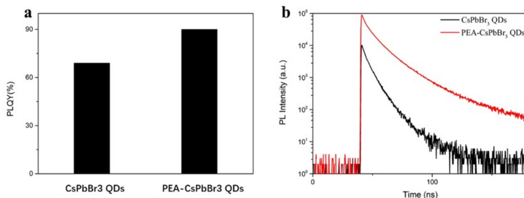
Figure S1. (a) PLQY measurements and (b) Time-resolved photoluminescence decay transient measurements of CsPbBr 3 QDs and PEA-CsPbBr 3 QDs.
