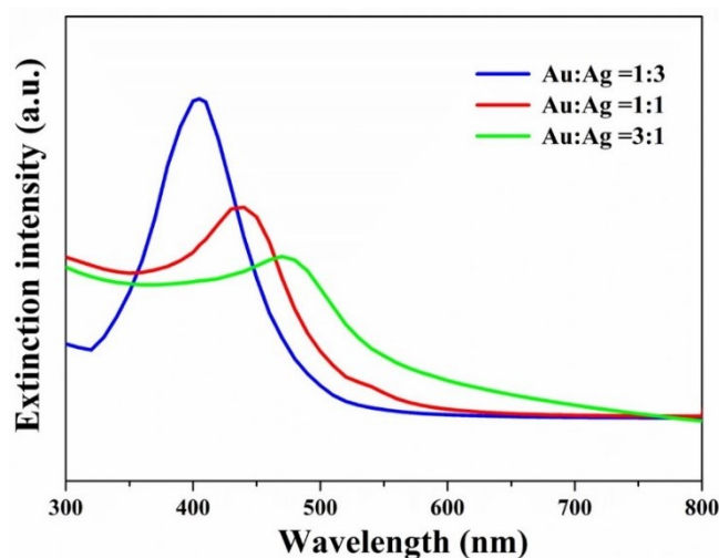
Fig. S2 The extinction spectra of \text{Au}_1\text{Ag}_3 ANPs, \text{Au}_1\text{Ag}_1 ANPs, and \text{Au}_3\text{Ag}_1 ANPs, corresponding to the blue, red, and green curves.
