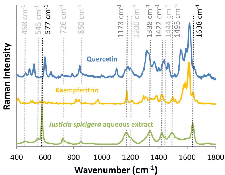
Figure S1. Conventional Raman spectra (532 nm) of the aqueous extract of Justicia spicigera leaves and of kaempferitrin and quercetin analytical grade molecules from Interchim (Montluçon, France)
