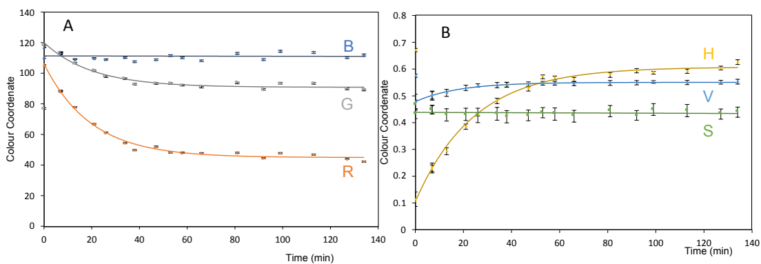
Figure S1. Colour co-ordinates versus time (min): A) RGB colour space; and B) HSV colour space.
