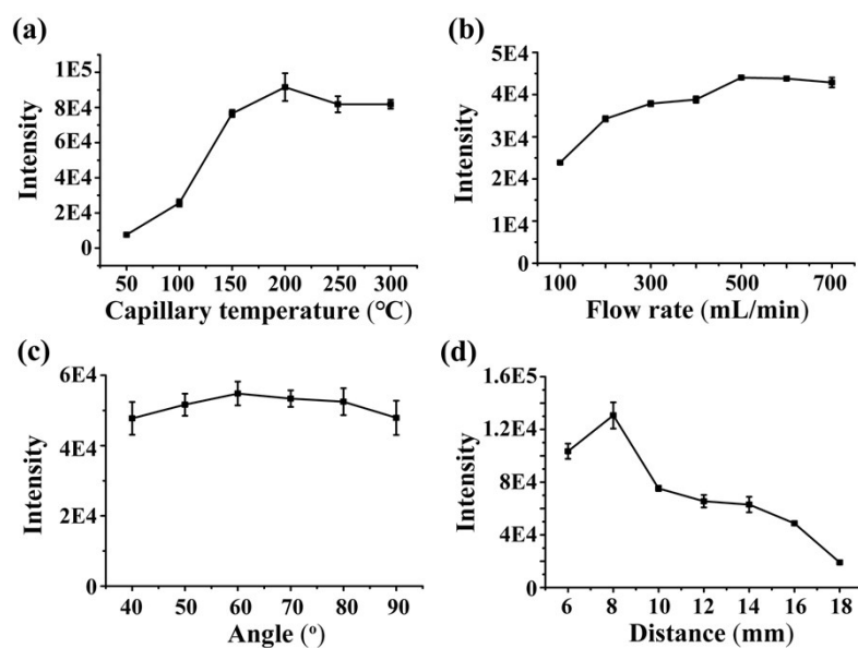
Fig. S3. Dependence of the m/z 76 signal intensity on working conditions in ambient corona discharge ionization MS. (a) Effect of the capillary temperature. (b) Effect of the flow rate of argon gas. (c) Effect of the angle between the tip of the peek tube and the tip of discharge needle. (d) Effect of the distance between the tip of the peek tube and the MS inlet.
