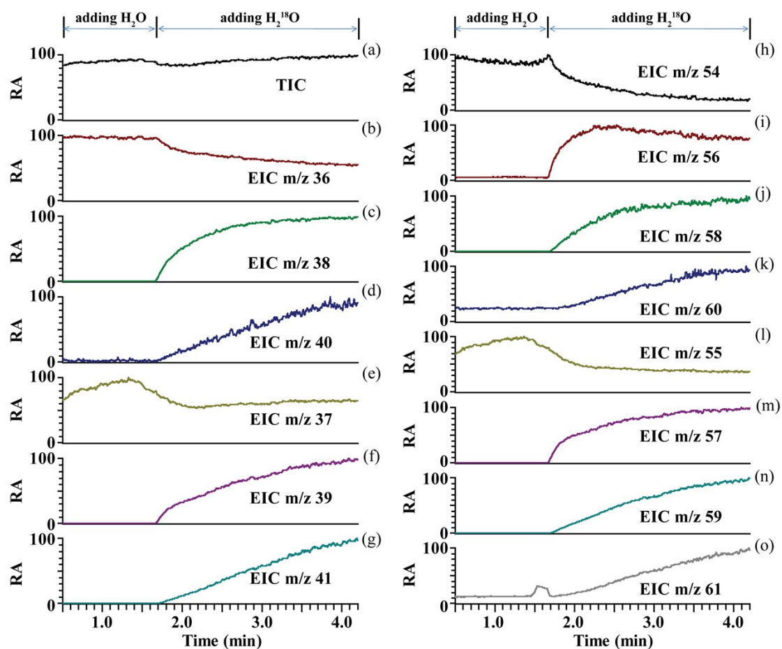
Fig. S4. The typical total ion chromatogram (TIC) and extracted ion chromatogram (EIC) of water related species when adding \text{H}_2\text{O} and \text{H}_2^{18}\text{O} by low energy ambient corona discharge ionization MS. (a) TIC, (b) EIC of m/z 36, (c) EIC of m/z 38, (d) EIC of m/z 40, (e) EIC of m/z 37, (f) EIC of m/z 39, (g) EIC of m/z 41, (h) EIC of m/z 54, (i) EIC of m/z 56, (j) EIC of m/z 58, (k) EIC of m/z 60, (l) EIC of m/z 55, (m) EIC of m/z 57, (n) EIC of m/z 59, (o) EIC of m/z 61.
