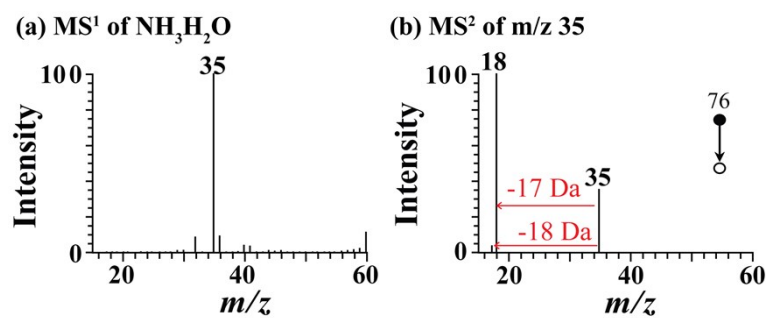
Fig. S5. Mass spectra of reaction between water radical cations and NH 3 . a) Typical mass spectrum showing [NH 3 + H 2 O] ++ formation. b) CID of ion of m/z 35 → products.
