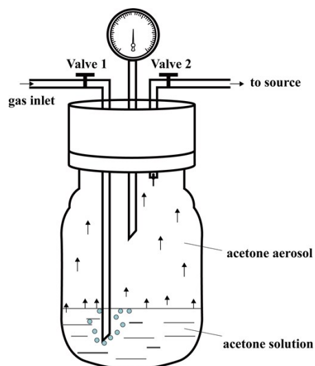
Fig. S1. The device used to the conversion of liquid phase concentration of acetone solution and gas phase concentration. The temperature of the container was 25 °C, and the pressure inside the flask was 1.1 \times 10^5 Pa.
