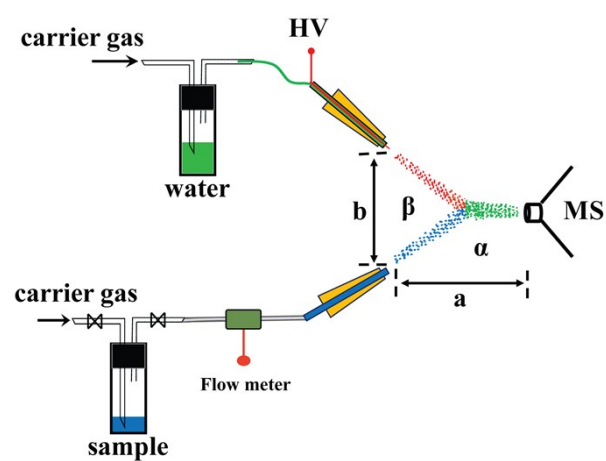
Fig. S2. Schematic illustration of acetone vapor analysis by low energy ambient corona discharge ionization mass spectrometry with (\text{H}_2\text{O})_2^{+*} as the extractive ionic reagent.
