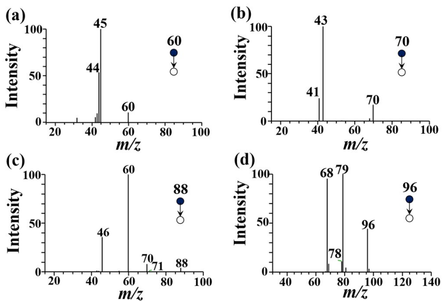
Fig. S8. CID-MS spectra of breath gas interacted with (H 2 O) 2 ++ by using ambient corona discharge ionization MS. (a) CID-MS spectrum of [trimethylamine + H] + at m/z 60. (b) CID-MS spectrum of [1-pyrroline + H] + at m/z 70. (c) CID-MS spectrum of [4-amino-butanal + H] + at m/z 88. (d) CID-MS spectrum of [benzene + H 2 O] ++ at m/z 96.
