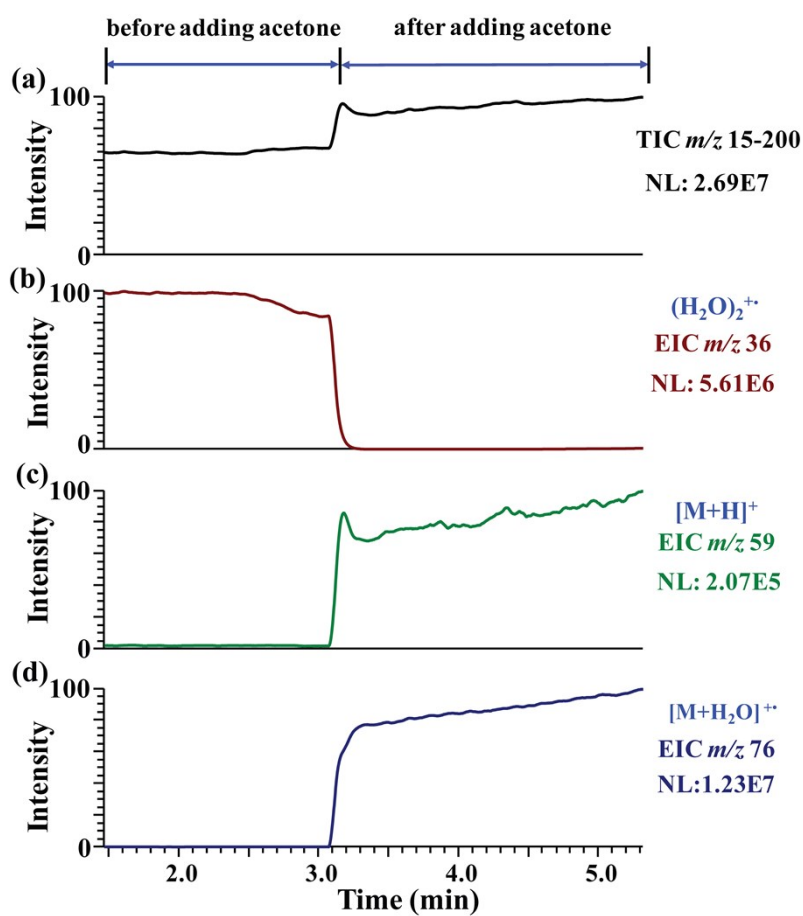
Fig. S6. The typical total ion chromatogram (TIC) and extracted ion chromatogram (EIC) of reaction between acetone and water radical cations by low energy ambient corona discharge ionization MS. (a) TIC, (b) EIC of m/z 36, (c) EIC of m/z 59, (d) EIC of m/z 76.
