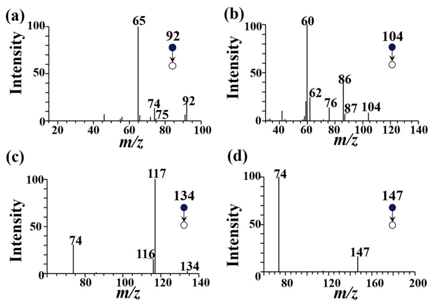
Fig. S9. CID-MS spectra of breath gas interacted with (\text{H}_2\text{O})_2^{++} by using ambient corona discharge ionization MS. (a) CID-MS spectrum of [propionic acid + \text{H}_2\text{O} ] ^{++} at m/z 92. (b) CID-MS spectrum of [2-pentanone + \text{H}_2\text{O} ] ^{++} at m/z 104. (c) CID-MS spectrum of [butyl acetate + \text{H}_2\text{O} ] ^{++} at m/z 134. (d) CID-MS spectrum of [2isoxazolidine + \text{H} ] ^{+} .
