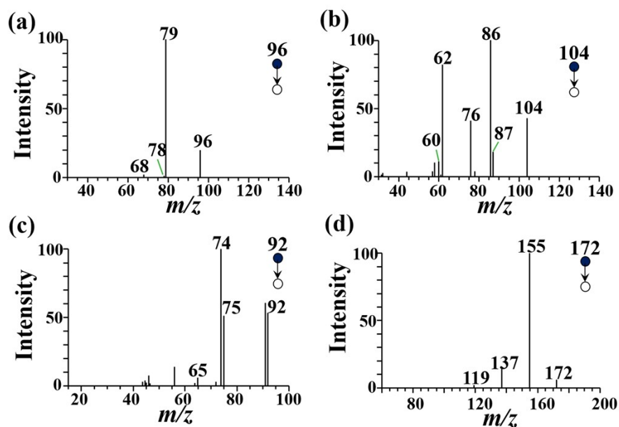
Fig. S7. CID-MS spectra of standards interacted with (\text{H}_2\text{O})_2^{++} by using ambient corona discharge ionization MS. (a) CID-MS spectrum of [\text{benzene} + \text{H}_2\text{O}]^{++} at m/z 96. (b) CID-MS spectrum of [\text{2-pentanone} + \text{H}_2\text{O}]^{++} at m/z 104. (c) CID-MS spectrum of [\text{propionic acid} + \text{H}_2\text{O}]^{++} at m/z 92. (d) CID-MS spectrum of [\text{bis(2-hydroxyethyl) disulfide} + \text{H}_2\text{O}]^{++} at m/z 172.
