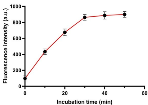
Figure S1. Fluorescence intensity of the sensing system with different incubation time of Cas12a enzyme.
