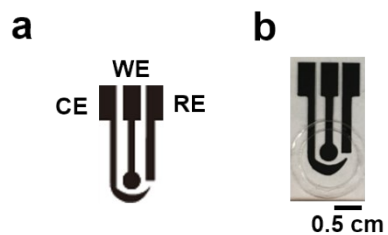
Figure S1. (a) Design drawing of a CSPE consisting of a reference electrode (RE), a working electrode (WE), and a counter electrode (CE). (b) Photograph of a completed CSPE with a ring-shape packing tape to confine the solution.
