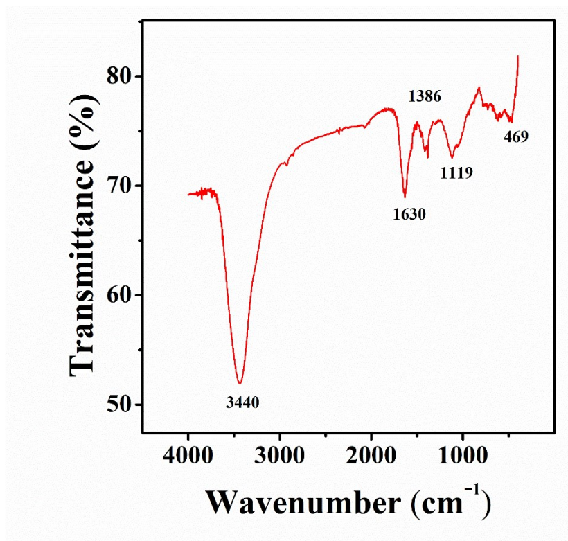
Figure S2. FT-IR spectrum of CHIT-MoS 2 QDs.
