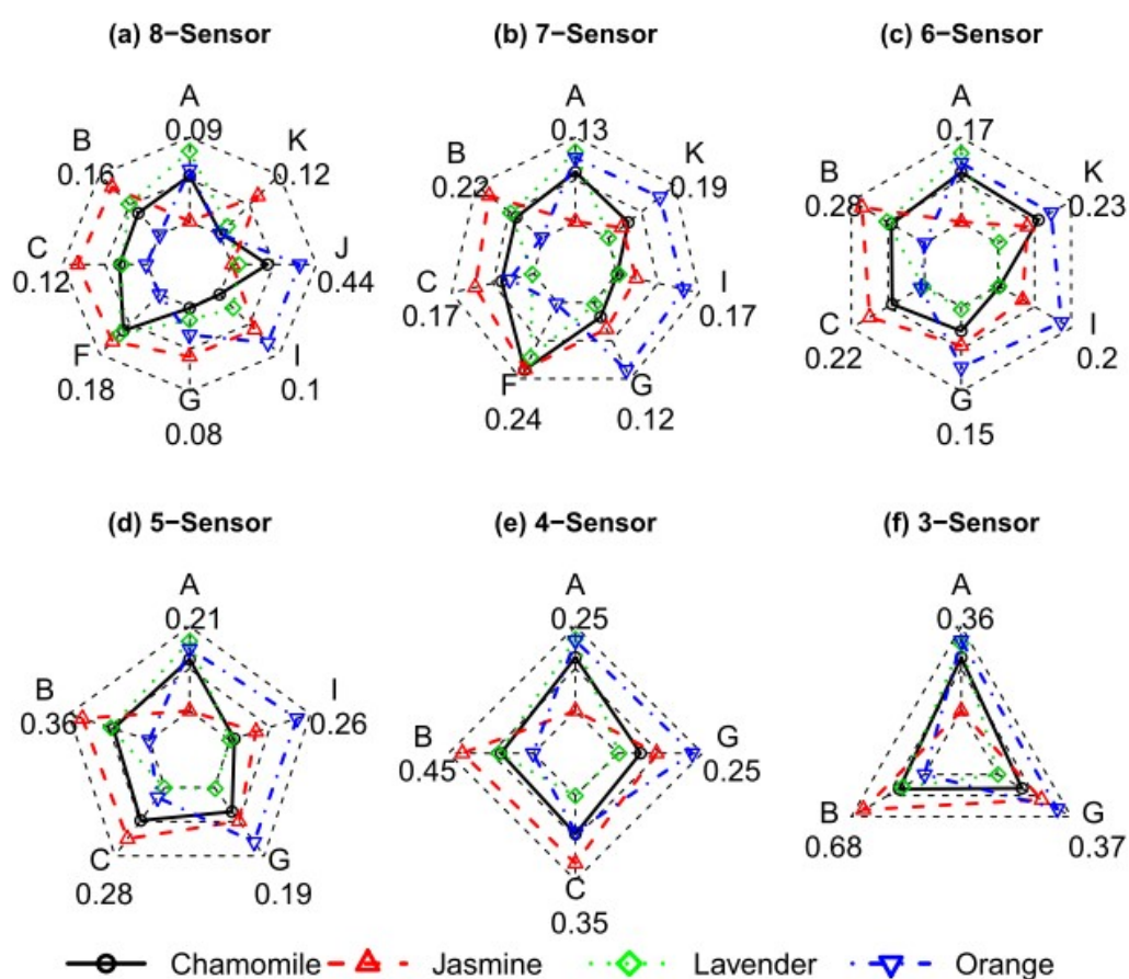
Fig S1 Radar chart of the normalized maximum response intensity to four aromas by arrays with different sensor numbers (with different axis ranges). (a) original array with all 8 sensors; (b) 7-sensor array without sensor J; (c) 6-sensor array without sensor J&F; (d) 5-sensor array without sensor J, F&K; (e) 4-sensor array with sensor A, B, C&G; (f) 3-sensor array with sensor A, B&G.
