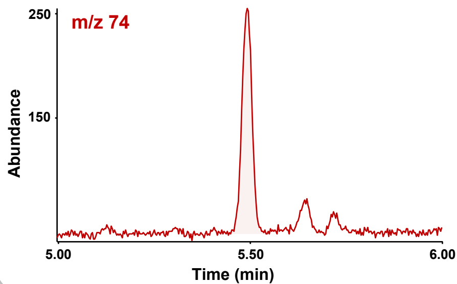
Fig. S1. Ion chromatograms of NDMA for (A) blank and (B) spiked samples
