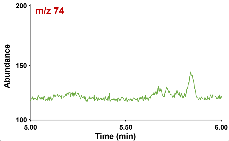
Fig. S1. Ion chromatograms of NDMA for (A) blank and (B) spiked samples
