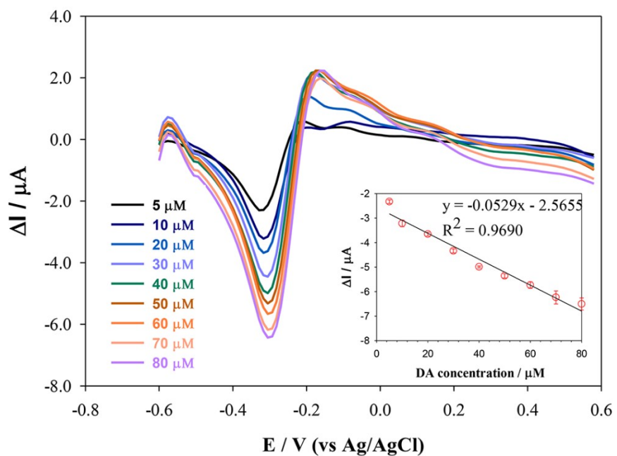
Figure S1. DPV curves of different DA concentrations (from bottom to top: 5, 10, 20, 30, 40, 50, 60, 70, 80 \mu\text{M} ) in a 0.1 M phosphate buffer solution at pH 7. RePNMA was used as the surface modifier on SPCE.
