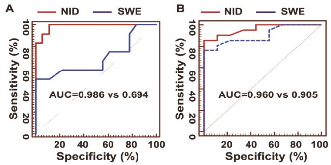
Fig S4
