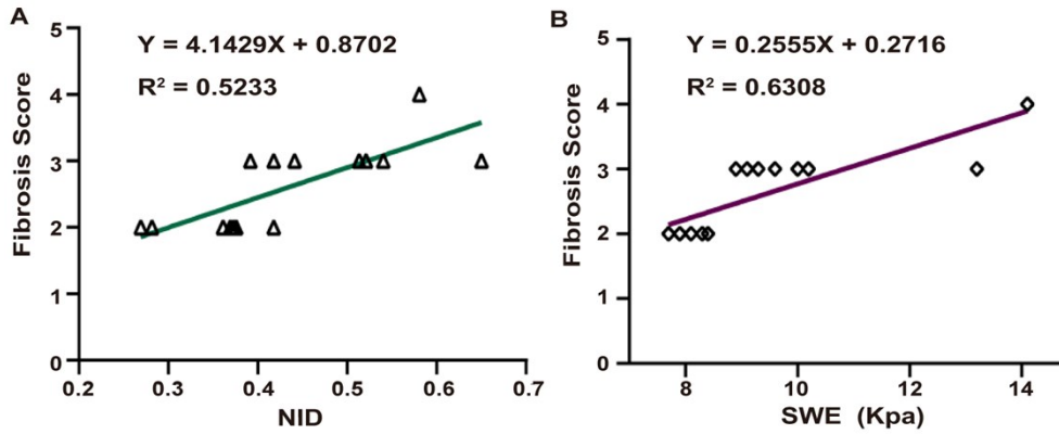
Fig S5
