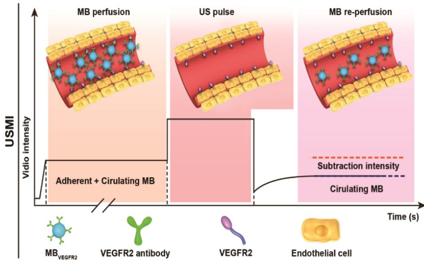
Fig S1
