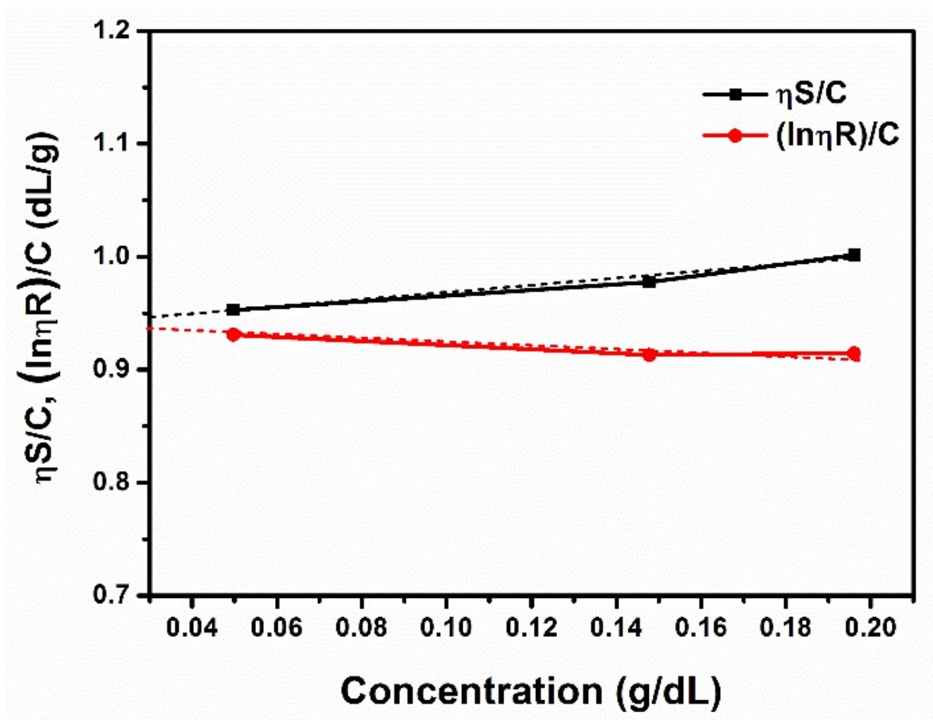
Figure S1: Determination of intrinsic viscosity of PLA
