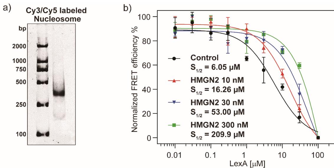
Figure S1. (a) The purity of Cy3/Cy5 labeled nucleosome for the FRET-based LexA titration experiments. (b) The LexA titration curves for nucleosomes incubating with different concentrations of unmodified HMGN2.
