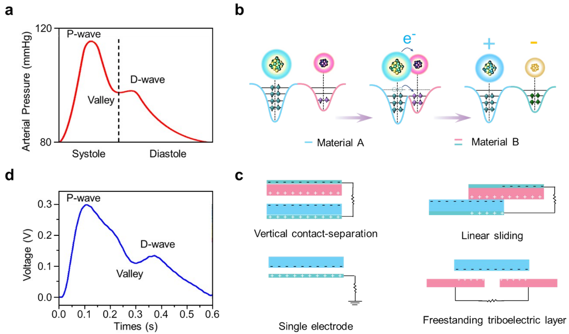
Fig. 2 Arterial pressure induced electricity generation via wearable TENGs for heart rate monitoring. (a and d) Comparison of pressure within large arteries during cardiac cycle with the voltage signals recorded during a respiration rate monitoring test, showing high reliability of TENG heart rate monitoring 46 . (b) The atomic-scale electron-cloud potential-well model of electricity generation via the conversion of biomechanical motions into electricity 39 . (c) The device-scale illustration of electricity generation.
