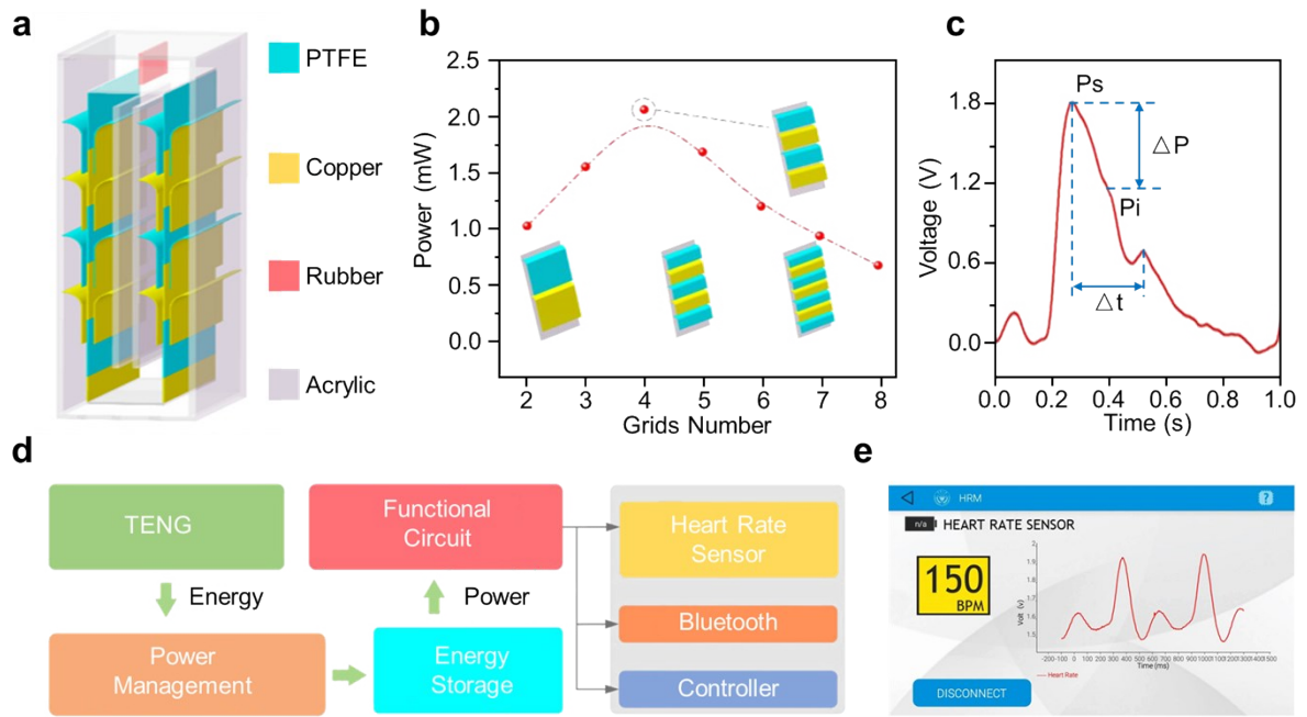
Fig. 5 TENGs as sustainable power sources for heart rate monitoring. (a) Schematic illustration of device structure of the D-TENG. (b) Output power of the D-TENG with different grid numbers under a consistent mechanical excitation of 10 Hz. (c) Heart-rate signal acquired by the BSN with an integrated D-TENG. (d) System diagram of the complete power-supplying system. (e) Enlarged view to show the whole software interface of the real-time acquired heart-rate signals 59 .
