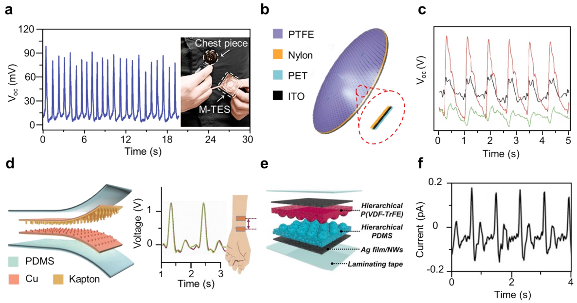
Fig. 3 Thin-film based TENGs as self-powered sensors for heart rate monitoring. (a) Output voltage signals of the M-TES as a heartbeat monitor, insert: setup of the M-TES as a heartbeat monitor 47 . (b) Schematic illustrations of the BMS. (c) The pulse waves acquired using BMS from three different sites of a participant: carotid artery, left wrist, and the chest 48 . (d) Schematic structure and radial artery pulse signal output generated by SUPS 33 . (e) Schematic illustration of humid-insensitive TESs wearing on the wrist. (f) Radial artery pulse waves detected by ultra-flexible TESs attached on the wrist 49 .
