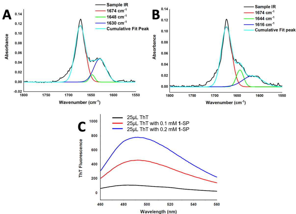
Figure S6. A) FT-IR spectra of a hydrogel of 1-SP formed at a concentration of 20 mM in water (90 mM TFA) with visible light irradiation at 22°C over 3 days. The gel was lyophilized then redispersed in D 2 O (20 mM) prior to recording the spectra. B) FT-IR spectrum of 1-SP formed at a concentration of 20 mM in water (90 mM TFA) with visible light irradiation at 60°C for 1 h. The gel was lyophilized then redispersed in D 2 O (20 mM) prior to recording the spectra. C) Fluorescence emission spectra of aqueous solutions of ThT (50 μM, PBS) with 0 (black), 1 (red) and 2 (blue) 5 μL aliquots of 1-SP hydrogel (formed at 10 mM, 22°C over 7 days) dispersed in ThT solution. The observed increase in emission at ~490 nm (440 nm excitation) indicates the presence amyloid-type nanofibers in the hydrogel.
