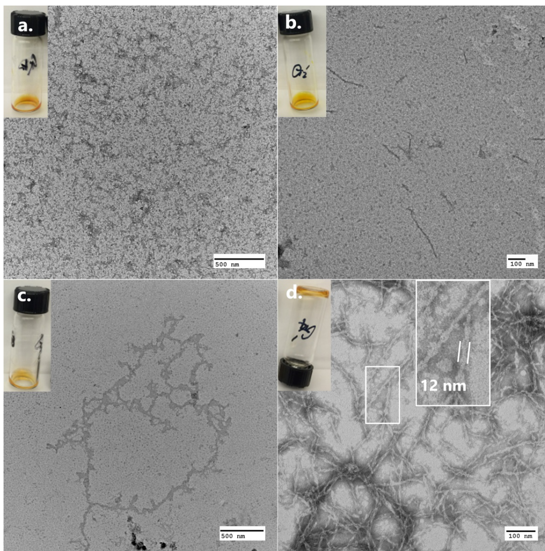
Figure S5. TEM images of aqueous solutions of 1 -SP (10 mM) under varying conditions. The solutions were heated to 60°C for 1 h to isomerize 1 -SP to 1 -MCH + , then incubated for 72 h at 22°C. A) in pure H 2 O (10 mM) under dark conditions ( 1 -MC); B) in aqueous TFA (90 mM) under dark conditions ( 1 -MCH + ); C) in pure H 2 O under visible light ( 1 -SP), and D) in aqueous TFA (90 mM) under visible light ( 1 -SP). Samples for TEM were prepared by diluting to 1 mM prior to imaging. Additional details about TEM experimental procedures are located above.
