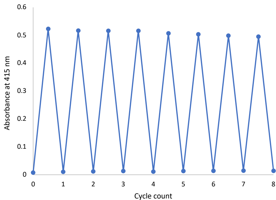
Figure S11. Photoswitching fatigue test on 1-SP (0.3 mM) in 90 mM TFA in water. One cycle consists of 60 min. of heating in dark at 60°C, followed by 5 minutes of visible light irradiation. A decrease of 4.7% in the maximum absorbance at 415 nm exhibited by the solution was observed after 8 cycles.
