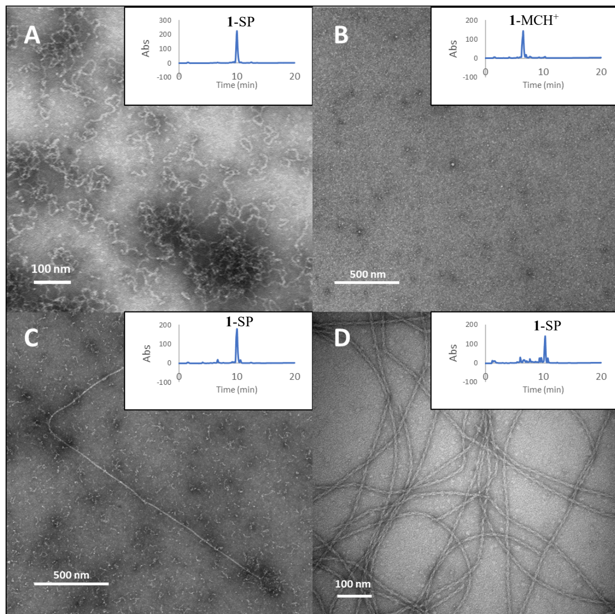
Figure S8. TEM images of 1-SP assembled in water (3 mM, 90 mM TFA, stained with uranyl acetate) at various time points. A) immediately after dissolution, showing initial aggregates, B) after 60 min at 60°C in the dark, showing the lack of any aggregates formed characteristic of 1-MCH + , C) after 30 min at 60°C with visible light irradiation showing longer fibers beginning to form, and D) after 24 h at 60°C with visible light irradiation showing a dense network of nanofibers. Graphical inserts show analytical reverse-phase HPLC traces (C8 reverse-phase column using a CH 3 CN/H 2 O 0.1% TFA gradient) of the samples used for TEM imaging.
