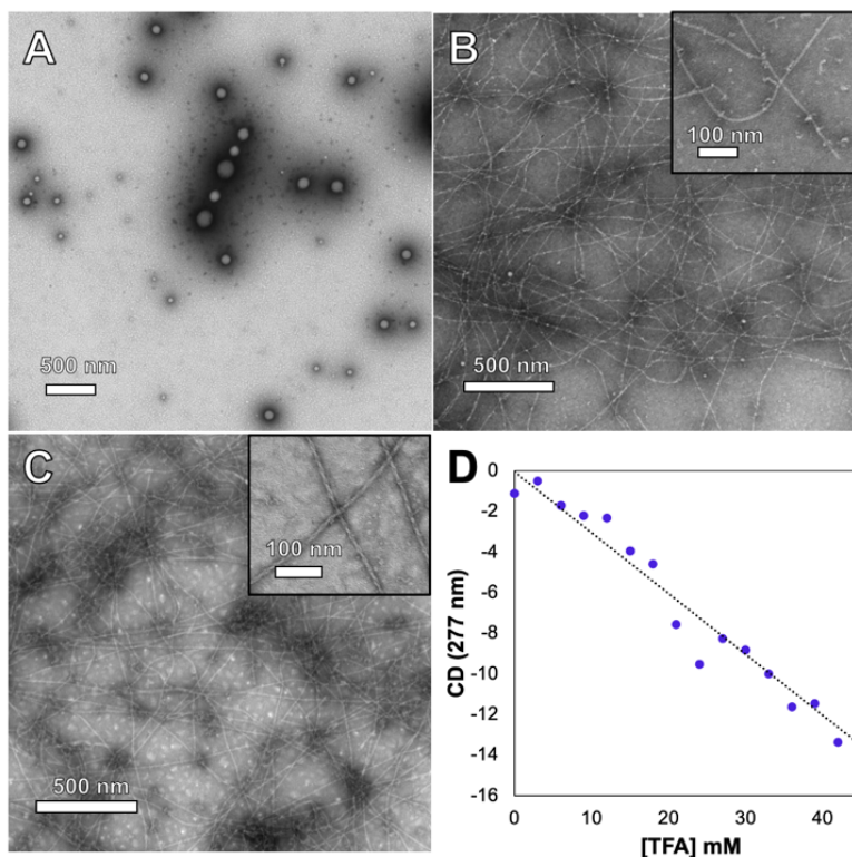
Figure S13. TEM images of 1 -SP (3 mM) in A) pure water, B) 13 mM TFA, and C) 90 mM NaTFA. D) Plot of CD signal at 277 nm of 1 -SP in water (3 mM) as function of TFA concentration, indicating progressively enhanced assembly. Samples of 1 -SP for each experiment were prepared under the dynamic self-assembly conditions (3 mM, 60°C, visible light).
