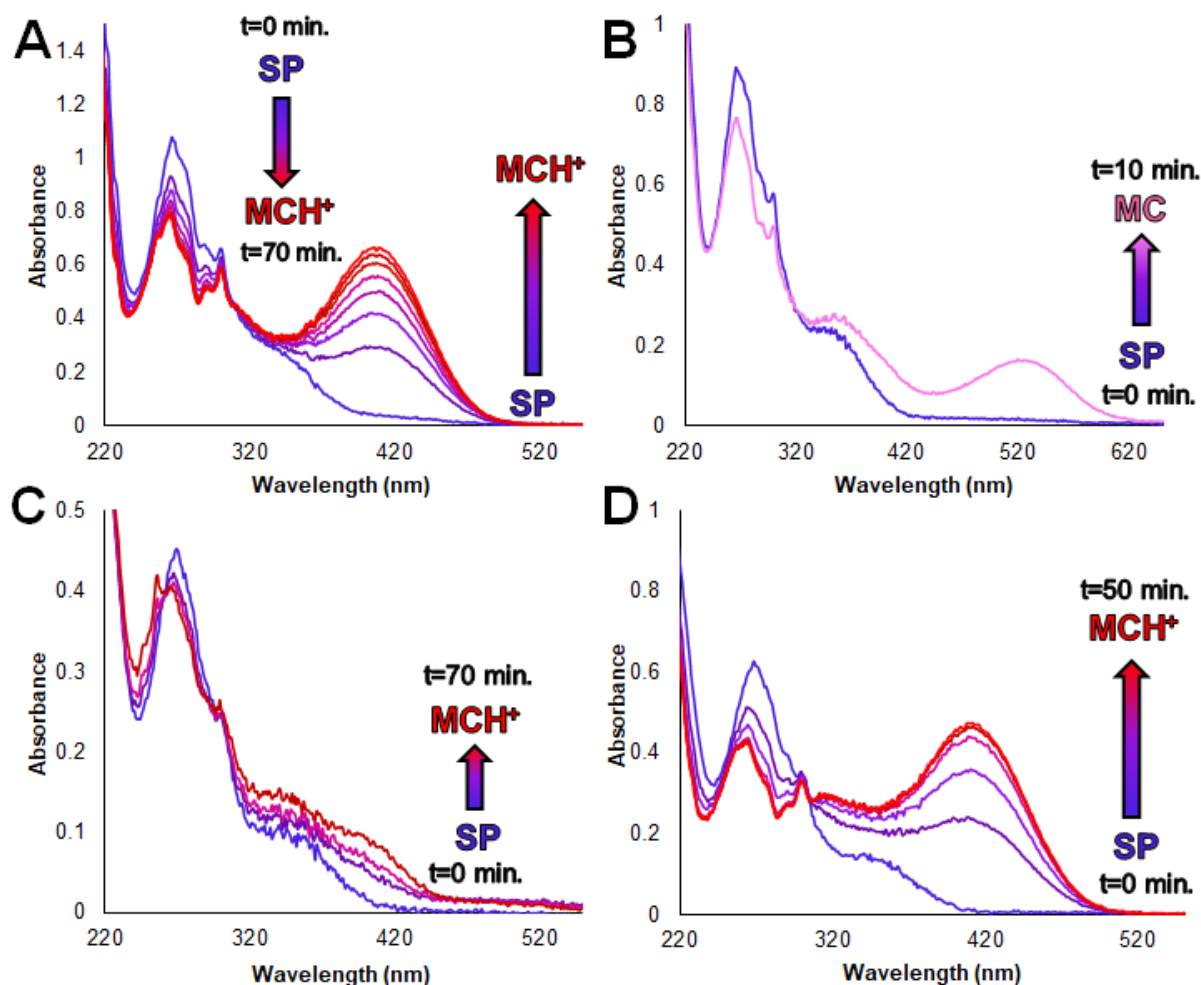
Figure S7. Thermal isomerization of 1-SP/1-MCH + . UV-Vis spectra showing 0.3 mM solutions of 1-SP at 60°C/darkness A) in CH 3 CN (90 mM TFA) showing an increasing concentration of 1-MCH + over 70 min, B) in pure water without added TFA, showing formation of small amounts of the unprotonated merocyanine form (1-MC) (purple to pink); C) in water with added NaCl (90 mM) showing little change over 120 min, and D) water/90 mM HCl showing conversion to 1-MCH + over 50 min.
