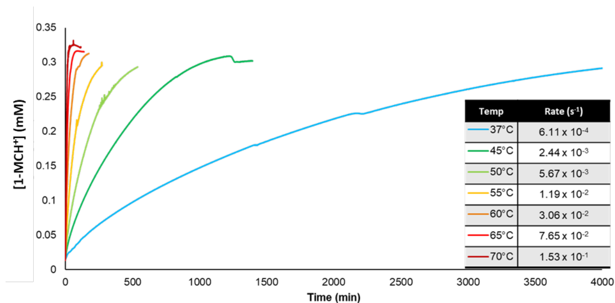
Figure S3. Plots of [1\text{-MCH}^+] versus time for 1-SP in water (0.3 mM, 90 mM TFA) at various temperatures. Concentration was determined by monitoring the 1\text{-MCH}^+ absorbance at 415 nm and converting the data to concentration using a standard curve. Rate constants were measured by fitting the change in [SP] concentration to a first order rate equation as described in the general methods.
