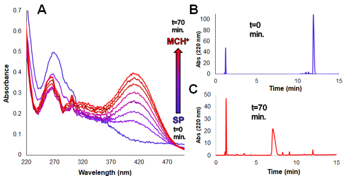
Figure S1. A) UV-Vis spectra of 1-SP (0.3 mM, 90 mM TFA in water) opening at 60°C/darkness over 70 min showing conversion from 1-SP to 1-MCH + , with corresponding reverse-phase analytical HPLC traces of the sample (C8 reverse-phase column using a CH 3 CN/H 2 O gradient) at B) 0 min and C) 70 min.
