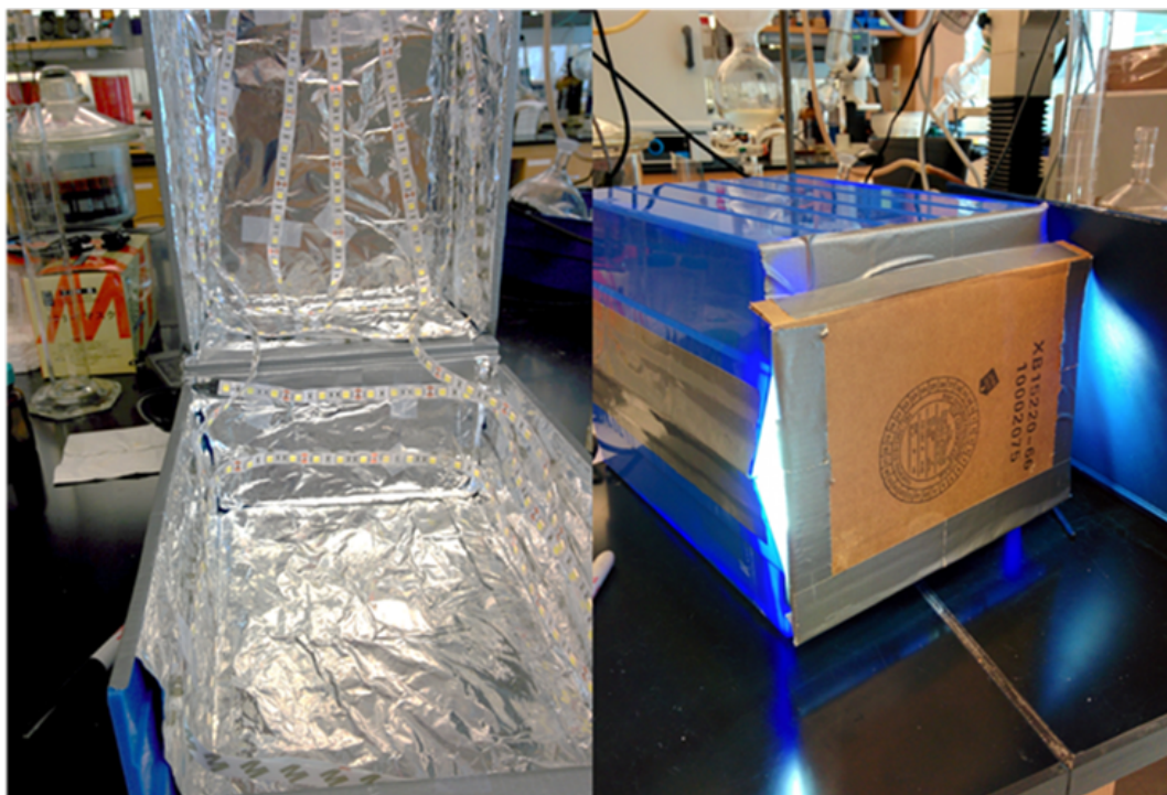
Figure S2. Experimental set-up for irradiation of 1-SP/MCH + samples. A strand of broad-spectrum white LED lights taped along the foil-lined top and sides of two polypropylene bins duct-taped together with a foil-lined cardboard opening. A small hot-plate/oil bath was placed inside for temperature-controlled experiments.
