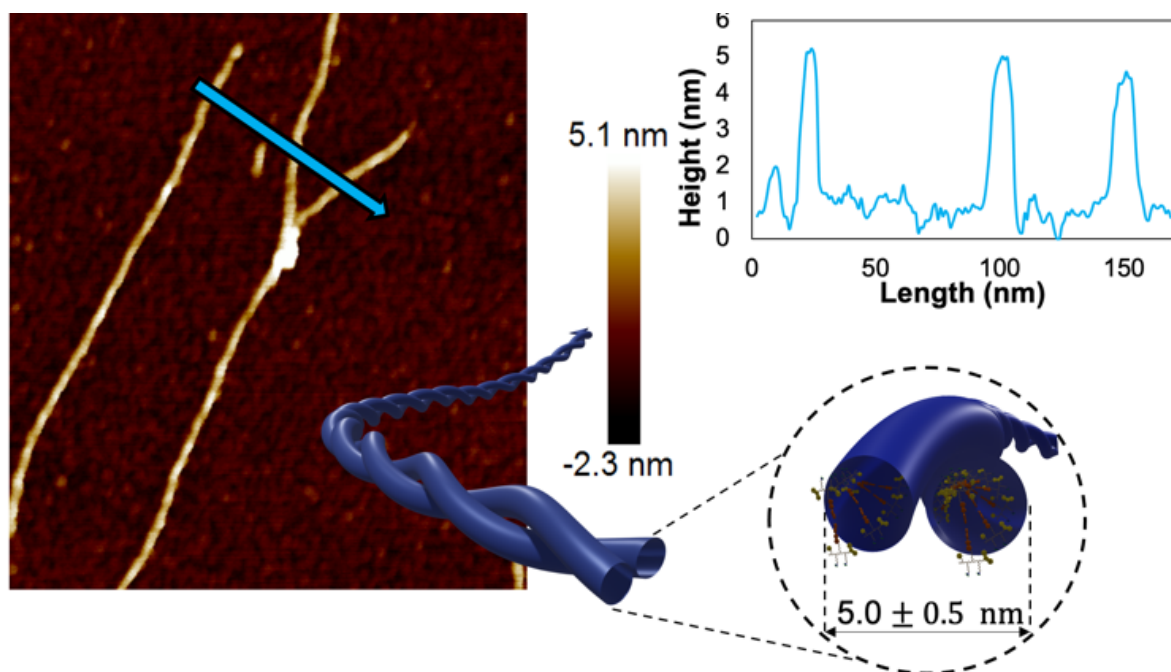
Figure S9. AFM images and height profiles of nanofibers of the hydrogel form by 1 form under dynamic conditions (60°C, visible light, 24 h).
