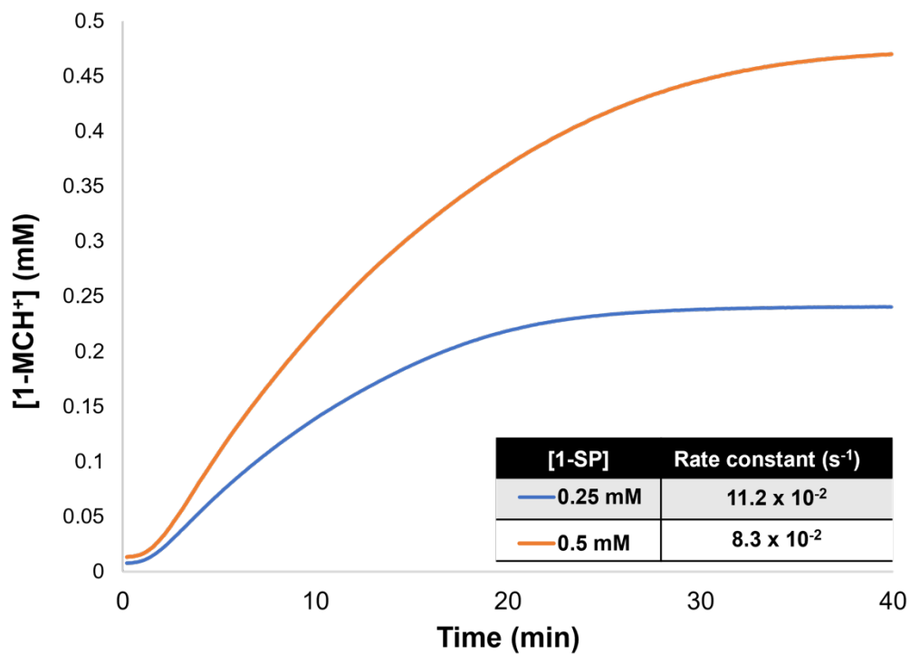
Figure S4. Plots of [1-MCH + ] versus time for 1-SP in water (65°C, 90 mM TFA) at 2 different concentrations. Concentration was determined by monitoring the 1-MCH + absorbance at 415 nm and converting the data to concentration using a standard curve. Rate constants were measured by fitting the change in [SP] concentration to a first order rate equation as described in the general methods.
