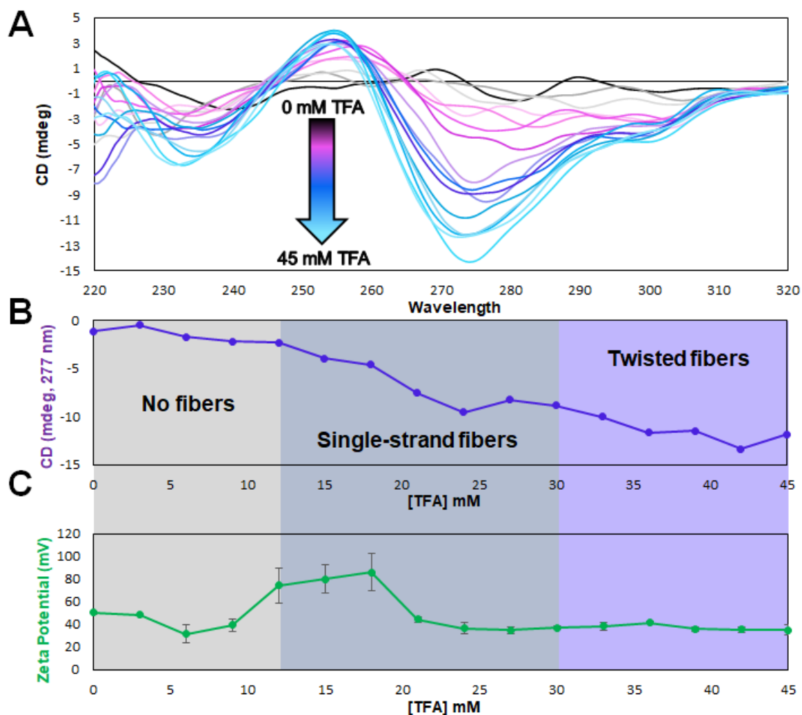
Figure S12. A) Self-assembly of 1 under dynamic conditions (4 h, 60°C, visible light, 3 mM 1 ) as a function of TFA concentration (0- 45 mM) showing an increase in the CD signal as the concentration of TFA increases; B) CD signal at 277 nm plotted against TFA concentration. C) Zeta potential (mV) as function of TFA concentration.
