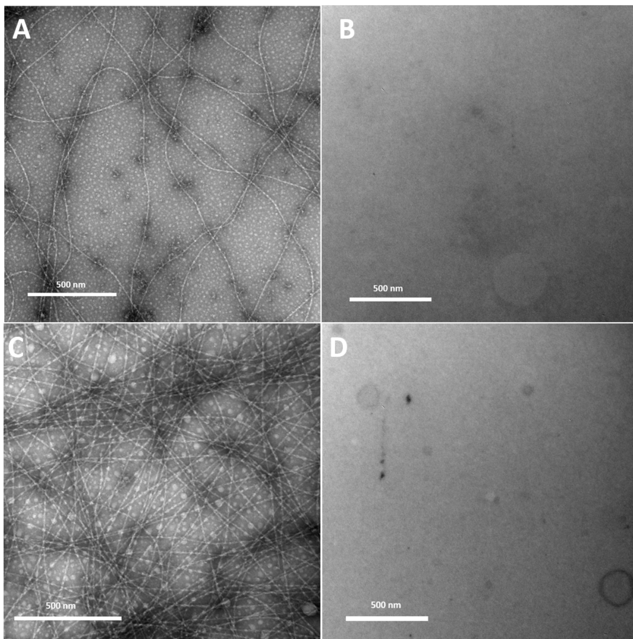
Figure S10. TEM images of 1-SP (3 mM) at 60°C in 90 mM TFA during on/off cycling of visible light (Figure 4). A) t=2 , 2 h of visible light, B) t=4 , light source turned off for 2 h, C) t=6 , 2 h of visible light, D) t=8 , light source turned off for 2 h.
