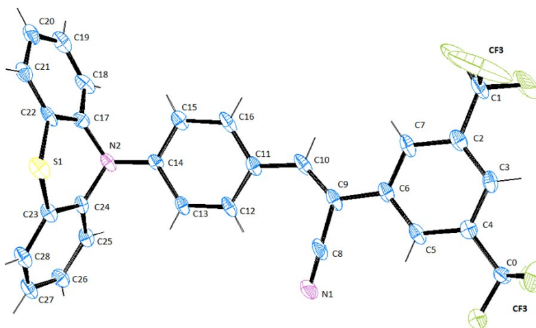
Figure S8. ORTEP view of PTX-2CF 3 with thermal ellipsoids shown at 30% probability.
