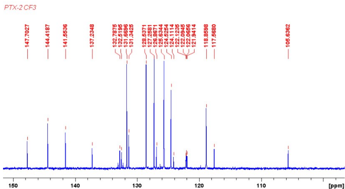
Figure S6. ^{13}\text{C} NMR spectra of molecule 1 in \text{CDCl}_3 ( C = 0.1 \text{ M} ).
