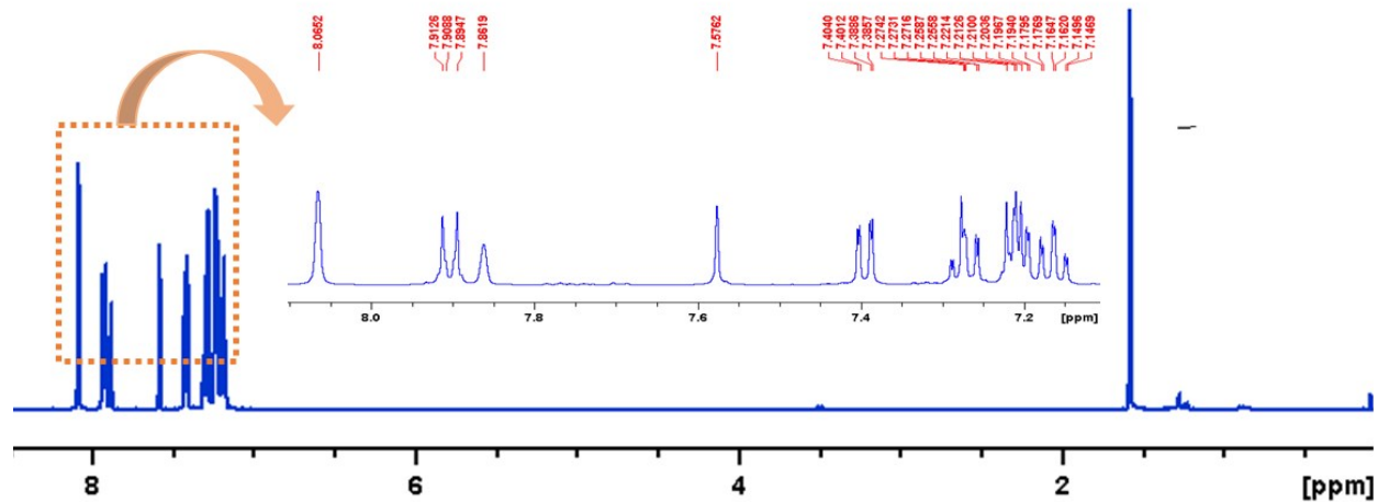
Figure S5. ^1\text{H} NMR spectra of molecule 1 in \text{CDCl}_3 ( C = 0.01 \text{ M} ).
