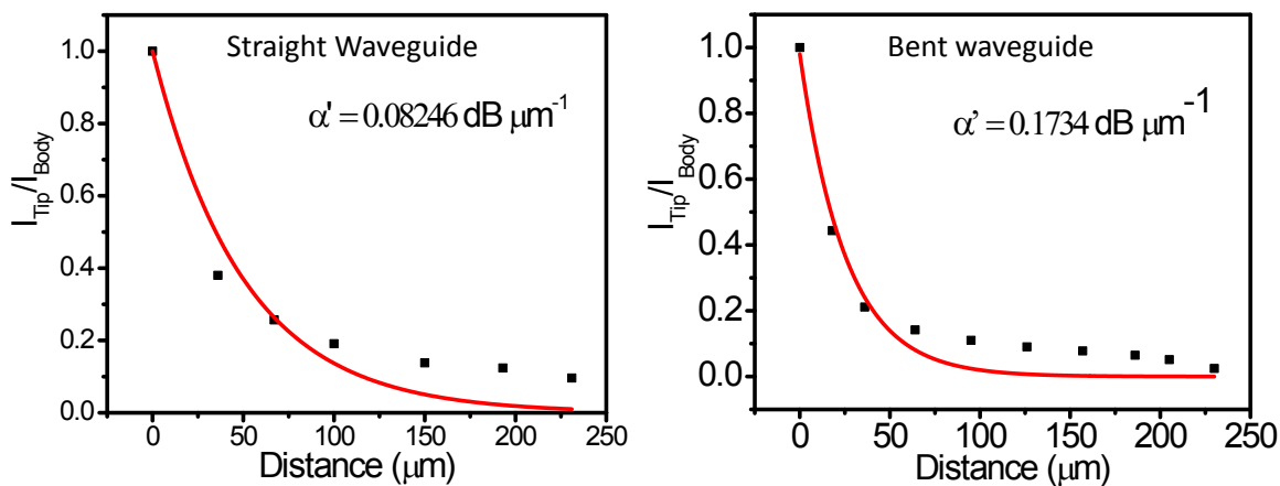
Figure S3. Optical loss fitting curves for straight and bent waveguides of PTX-2CF 3 .
