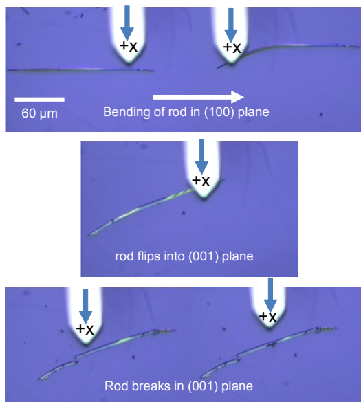
Figure S1. Flexibility of crystal in various planes when force is applied in perpendicular direction.
