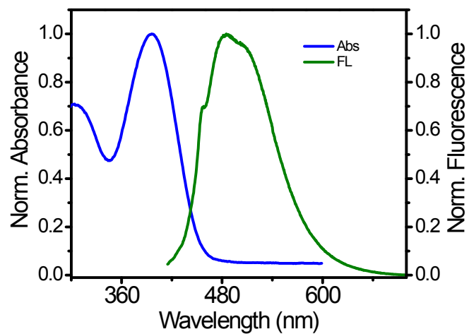
Figure S9. Normalized Absorbance and emission of PTX-2CF 3 in THF solution ( C = 1.2 \times 10^{-5} mM).
