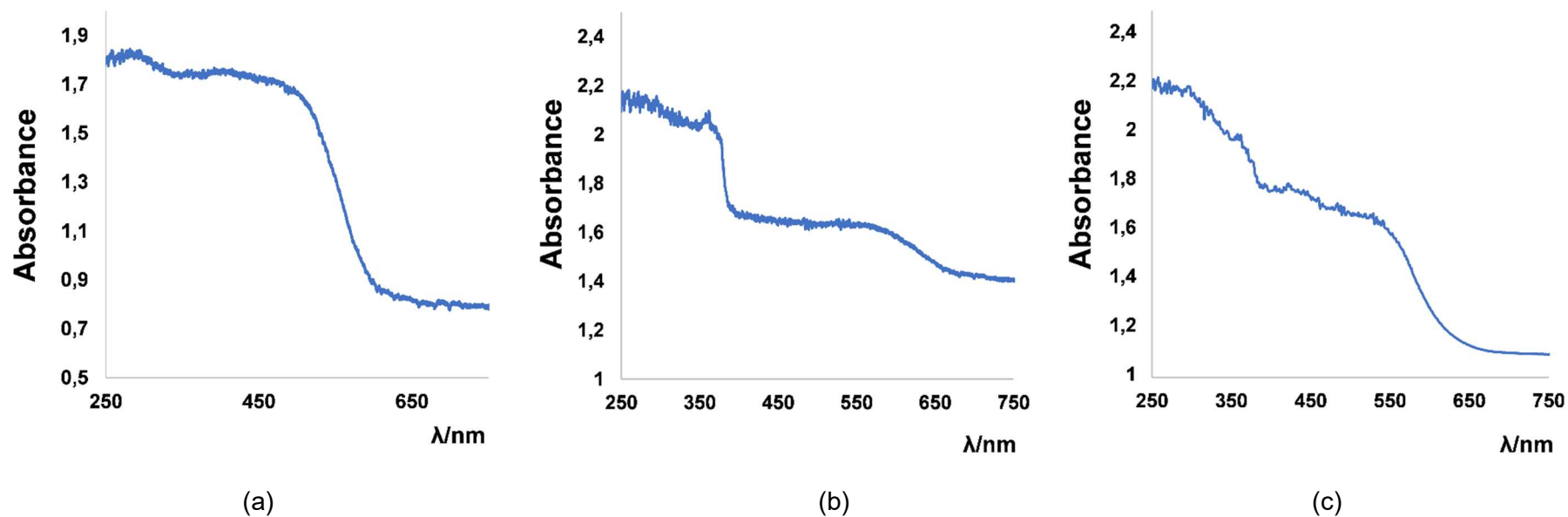
Figure 1. a) Solid state UV-Vis spectra of (a) 2 , (b) 2 Hm , and (c) 2 ow recorded on a Thermo Scientific Evolution 350 UV-Visible Spectrophotometer.
