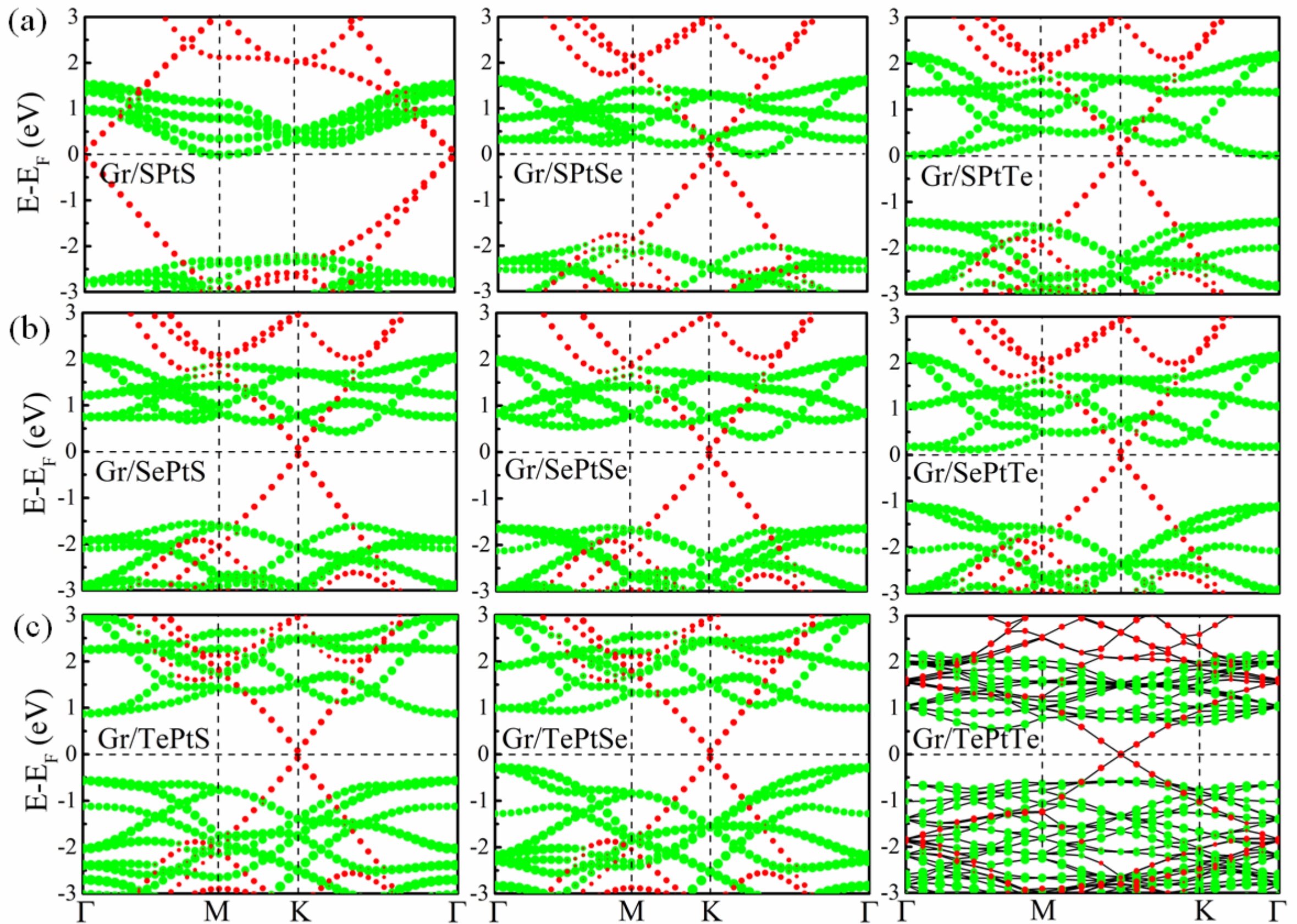
Fig. S1 The projected band structures of the Gr/XPtY systems based on HSE06 hybrid functional method. The green and red lines stand for the contribution of XPtY layer and Gr, respectively. (a) The Gr/SPtY systems. (b) The Gr/SePtY systems. (c) The Gr/TePtY systems..
