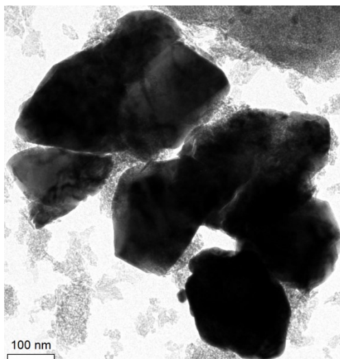
Figure S1 TEM-image for Bi/Al 2 O 3 sample
