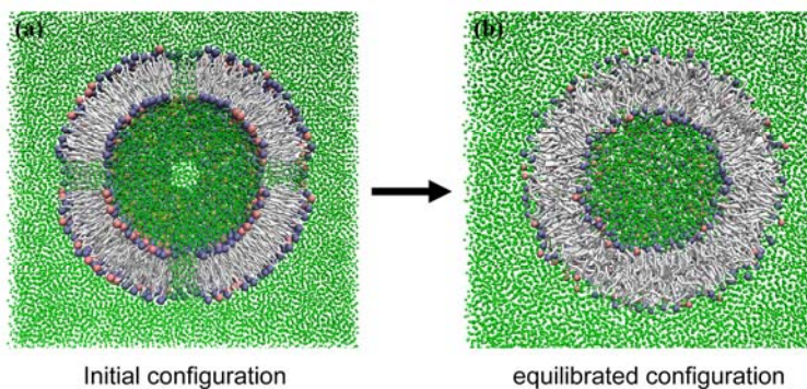
Fig. S1. The (a) initial and (b) final equilibrated configurations of the lipid vesicle.
