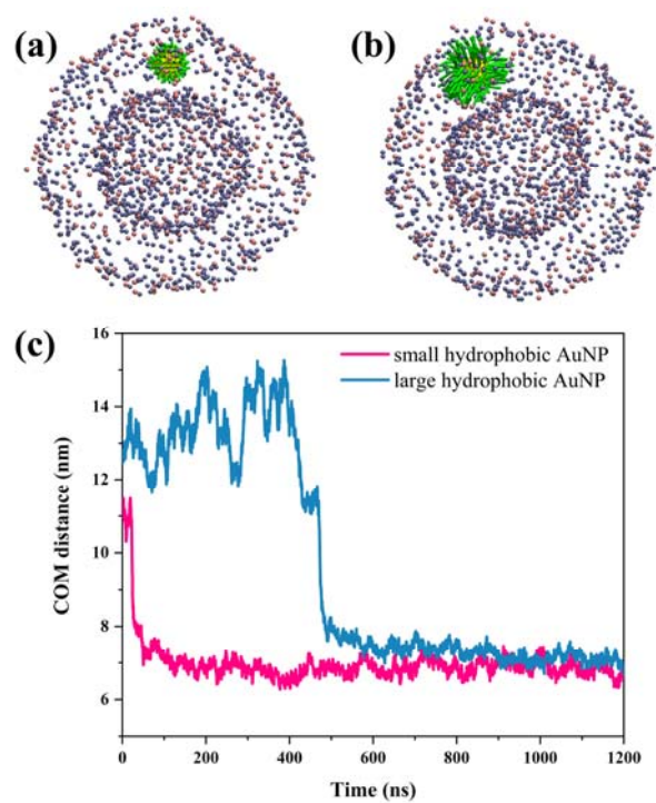
Fig. S2. Equilibrated states of (a) small and (b) large hydrophobic AuNPs interacting with the lipid vesicle, (c) COM distance between hydrophobic AuNPs and the lipid vesicle.
