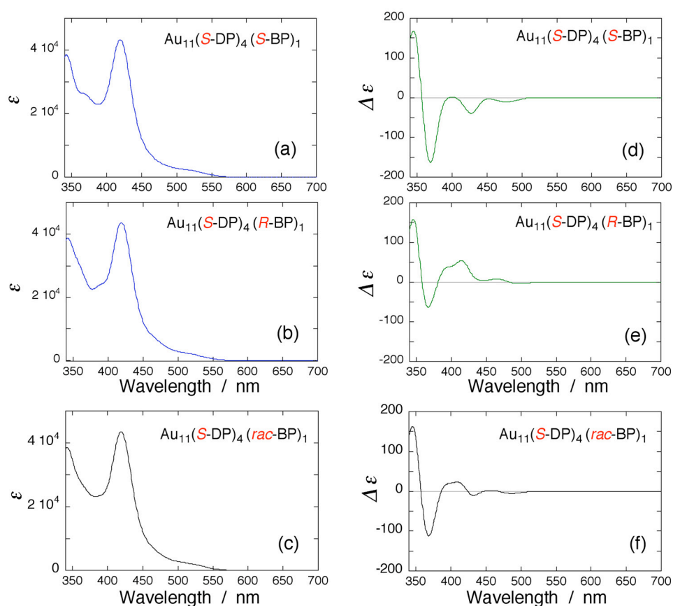
Fig. S1. Simple average of absorption ((a) or (b)) and CD spectra ((d) or (e)) of isomers 1_{\text{S}}\text{--}5_{\text{S}} or 1_{\text{R}}\text{--}5_{\text{R}} , respectively. (c) or (f) shows absorption or CD spectrum that can be obtained as a simple average of (a) and (b), or (d) and (e), respectively.
