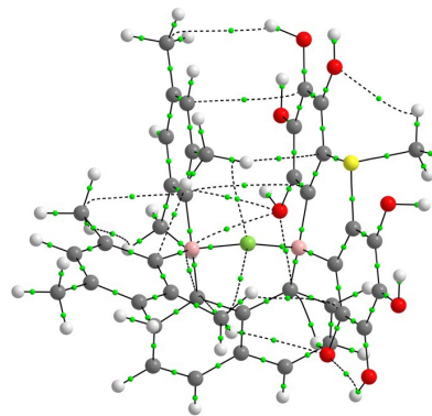
4\text{NO}_2\cdots\text{F}^-
