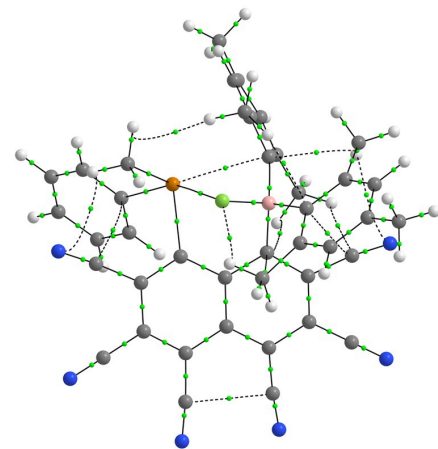
4\text{CN}\cdots\text{F}^-
