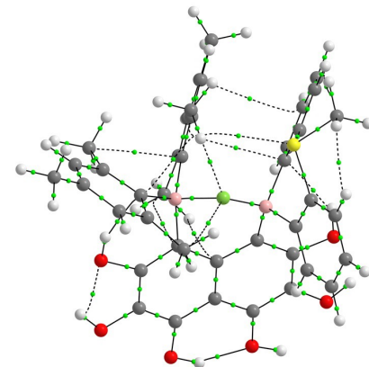
5\text{H},\text{OH}\cdots\text{F}^-
