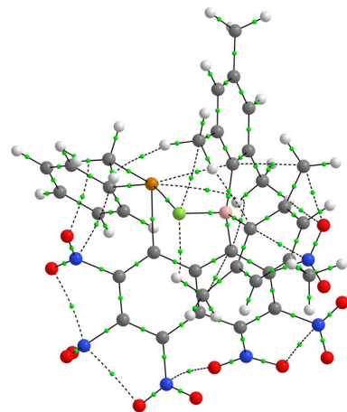
4\text{NO}_2\cdots\text{F}^-
