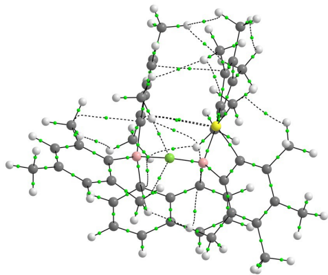
5\text{CH}_3,\text{H}\cdots\text{F}^-
