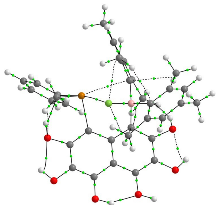
4\text{OH}\cdots\text{F}^-
