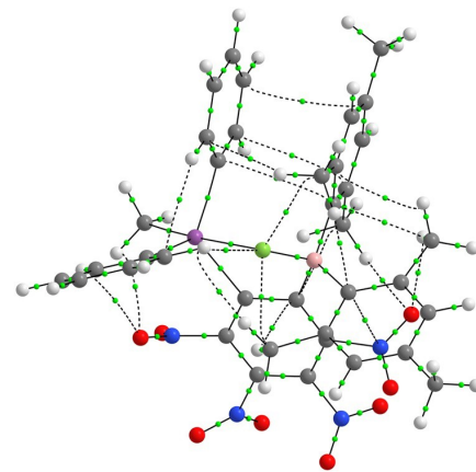
5\text{CN}, \text{H}\cdots\text{F}^-
