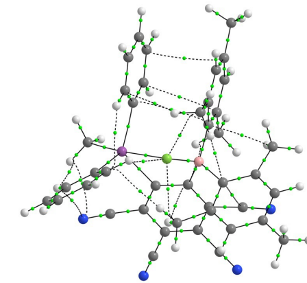
5\text{H}, \text{CN}\cdots\text{F}^-
