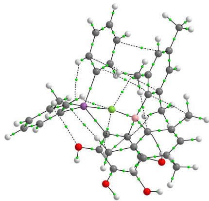
5\text{H}, \text{NO}_2\cdots\text{F}^-
