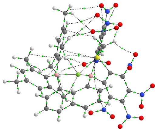
5\text{NO}_2, \text{H}\cdots\text{F}^-
