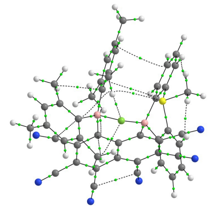
5\text{H}, \text{CN}\cdots\text{F}^-
