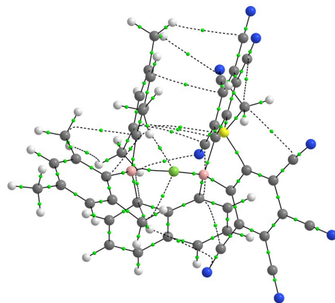
5\text{CN}, \text{H}\cdots\text{F}^-
