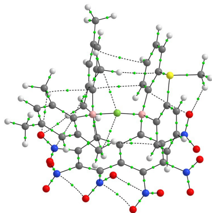
5\text{H}, \text{NO}_2\cdots\text{F}^-
