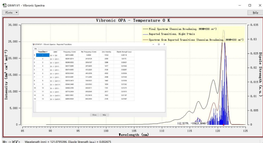
Figure S2. The calculated Franck-Condon factors and the simulated photoelectron spectrum.
