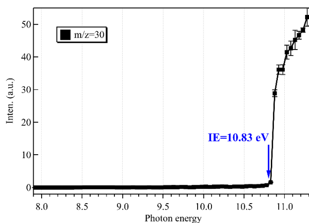
Figure S1. Photoionization spectrum of m/z = 30 .
